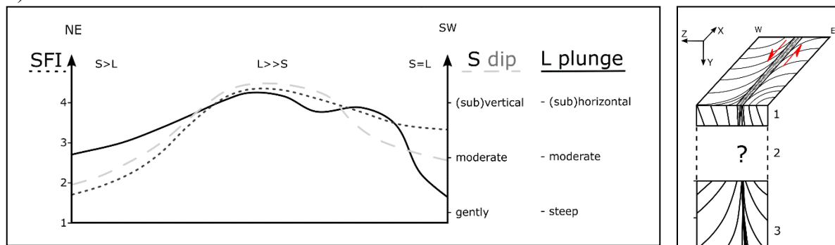
Figure 3 (top). Diagram of the central segment of the Kynsikangas shear zone displaying shape fabric intensity (SFI), foliation (S) and lineation (L). We note a correlation in strain intensity, geometry and orientation of mineral fabrics.
