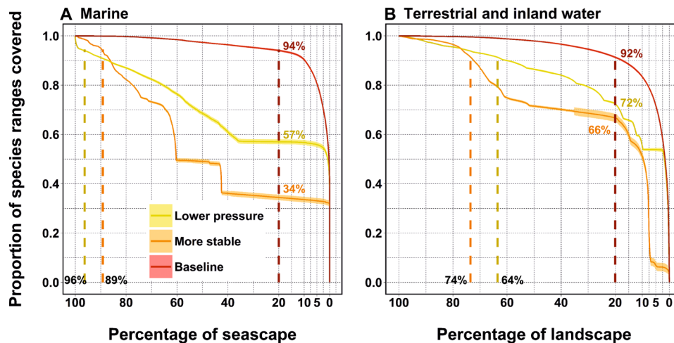
Fig. 3. Average representation for 4543 species threatened by unsustainable commercial harvesting at each percentage of the seascape and landscape. Curves quantify the proportion of the species' ranges represented at each percentage of the seascape (A) and landscape (B) under different scenarios. "Baseline" curves show representation when only species range maps were included in the analysis. "Lower pressure" is for the scenario in which maps of accessibility and fisheries catch were additionally included in the analysis as cost layers to implement avoidance of areas with high-threat intensity. "More stable" curves are for analysis in which the Fragile State Index was included as a cost layer to implement avoidance of areas where the rule of law is lowest. The red dashed vertical line shows species representation at the top 20% ranked areas. Yellow and orange dashed lines show the percentage of landscape and seascape needed to achieve same species representation as in the baseline scenario under the lower pressure and more stable scenarios, respectively. Black numbers report the percentage of landscape and seascape needed to achieve such representation. Red, yellow, and orange numbers show mean species representation within the top 20% ranking areas under the baseline, lower pressure, and more stable scenarios, respectively.
