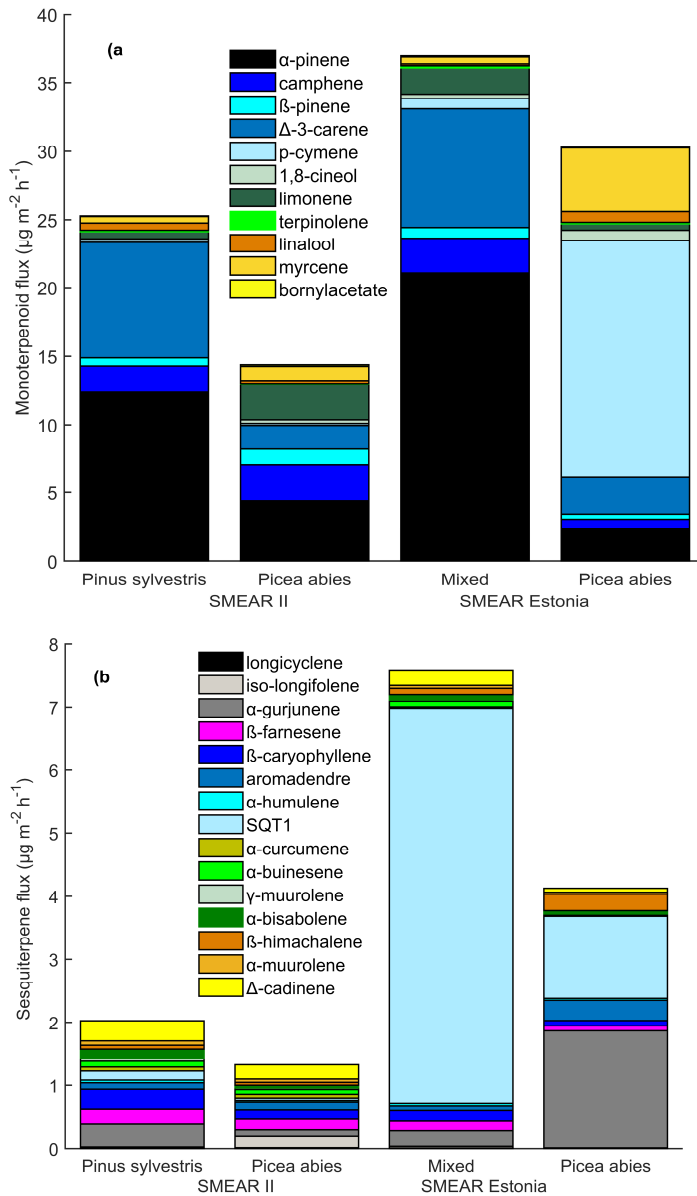
Figure 8. Individual mean monoterpenoid and sesquiterpene fluxes ( \mu\text{g m}^{-2} \text{h}^{-1} ) from Pinus sylvestris and Picea abies forest floors in boreal (SMEAR II) and from mixed and Picea abies forest floors in hemiboreal (SMEAR Estonia) climates in 2017–2018 (study II).
