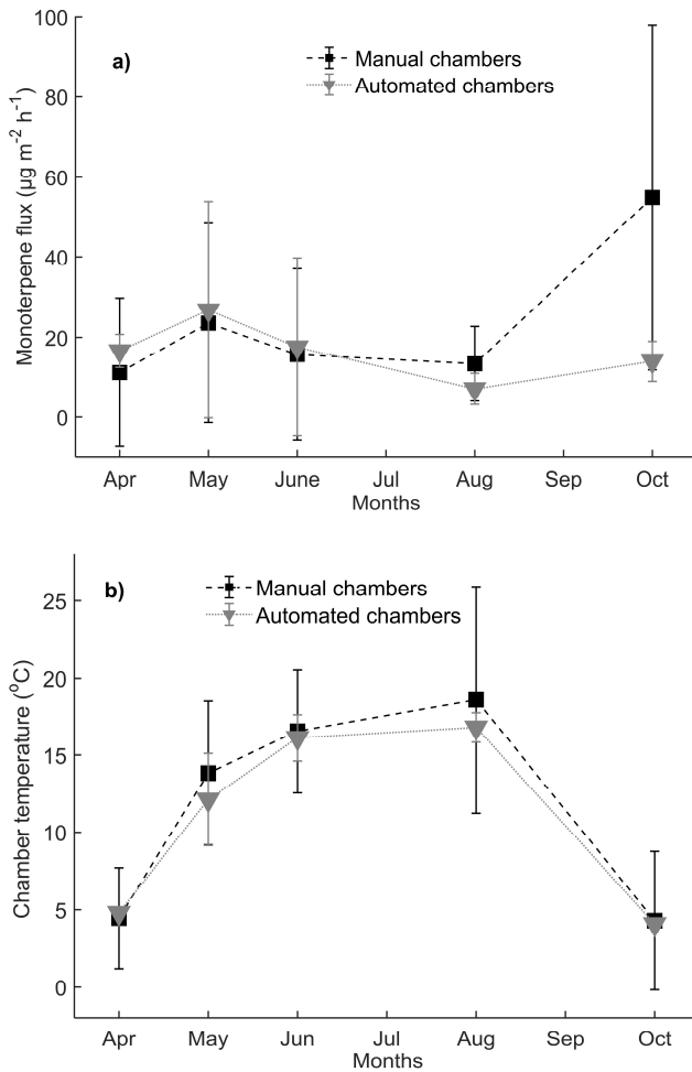
Figure 13. Monthly mean (a) monoterpene fluxes and (b) chamber temperature ( ^{\circ}\text{C} ) from a boreal forest floor measured using automated chambers ( n = 3 ) connected to the quadrupole-PTR-MS and manual chamber measurements ( n = 4\text{--}9 ) quantified using the TD-GC-MS in 2015. Monoterpene flux measurements using automated chambers were performed simultaneously with the manual chamber measurements. Error bars are the standard deviation of the chambers for each month.
