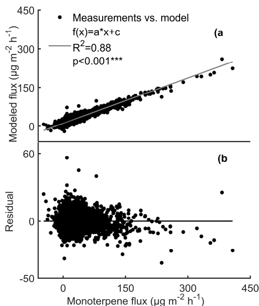
Figure 12. Comparison between measured monoterpene fluxes (µg m -2 h -1 ) (a) from the forest floor and fluxes calculated using the mixed effects linear model with linear fit and (b) residuals (study I). The model is based on the flux data measured from all three chambers between 2010 and 2017 (modified based on Mäki et al., 2019). Grey line: measured flux = modeled flux.
