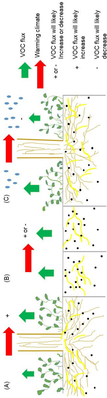
Figure 1. The possible direct effects (+ or - = total VOC flux will increase or decrease, + = total VOC flux will likely increase and - = total VOC flux will likely decrease) of the warming climate (red arrow) on total VOC fluxes (green arrow) from northern soils. (A) Higher temperature increases VOC biosynthesis of plants and VOC release from leaves. (B) Higher temperature increases microbial activity = VOC synthesis and uptake of microbes. (C) Heavy rain increases soil moisture and hinders gas diffusion in soil and VOC evaporation from the soil surface.
