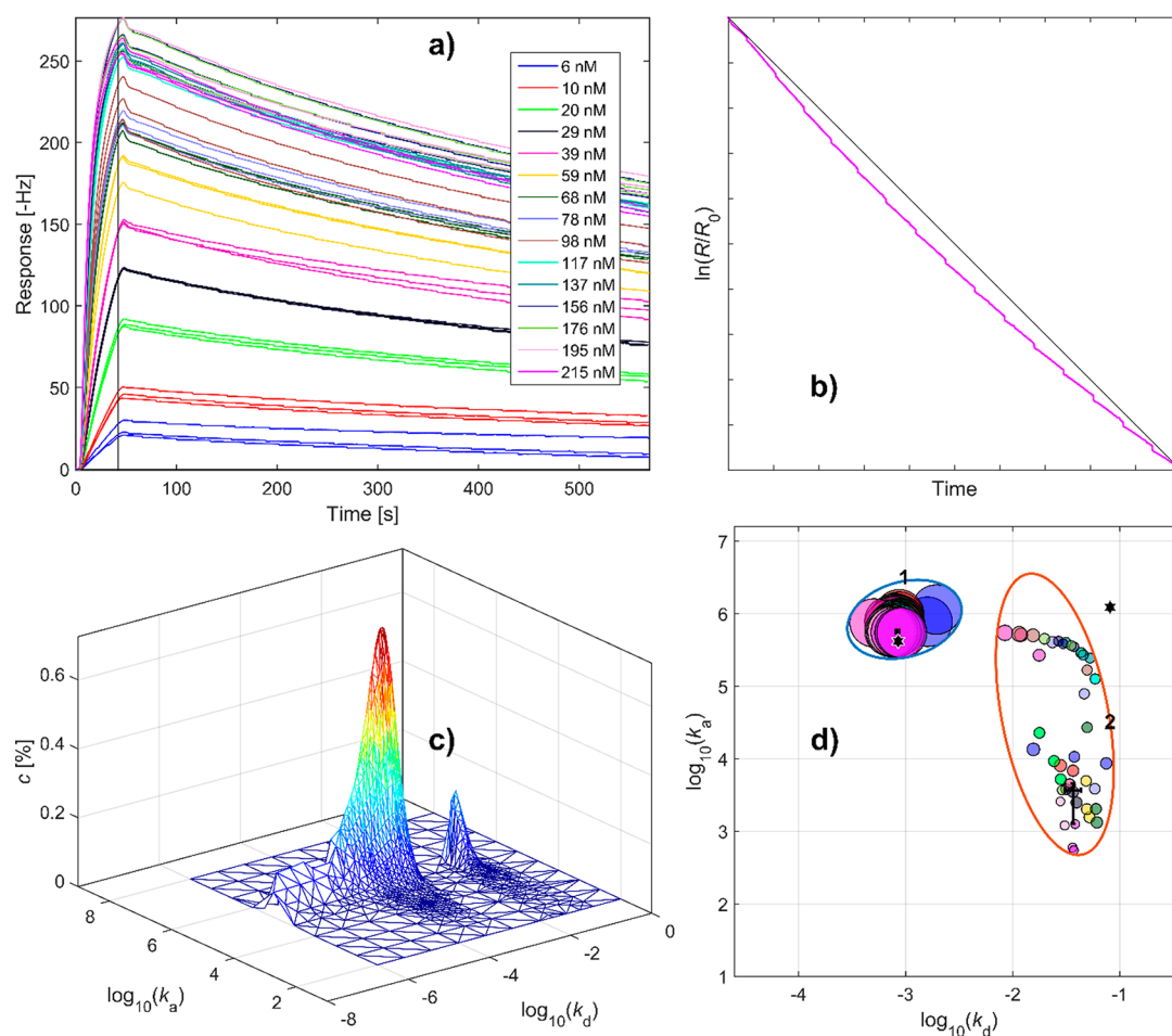
Figure 3. (a) Sensorgrams for an IDL-VLDL-anti-apoB-100 system at different analyte concentration levels. (b) Dissociation graph for a 215 nM injection. (c) Rate Constants Distribution (RCD) for a 20 nM injection. (d) Rate constants obtained by fitting a two interactions model to the sensorgrams one by one. See Figure 1 for more details and the Supporting Information Table S3 for rate constants.
