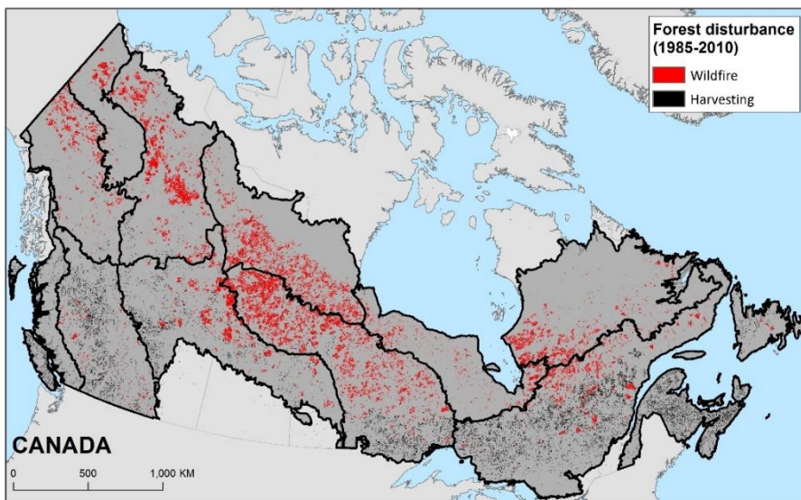
Figure 13. Area disturbed by wildfire and harvest in Canada's forested ecosystems (1985–2010).
