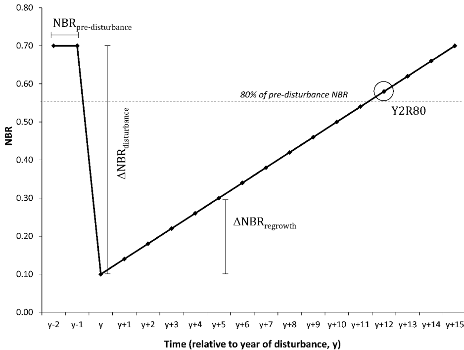
Figure 9. A schematic of a spectral NBR pixel series illustrating the short-term spectral recovery absolute ( NBR_{regrowth} ) and relative (Recovery Indicator, RI) metrics and the long-term spectral recovery metric, Y2R.
