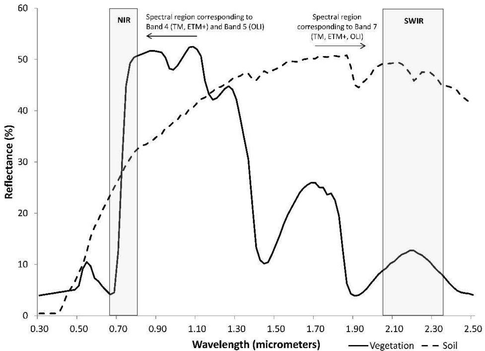
Figure 2. Spectral profiles of vegetation and soil with the near infrared (NIR) and shortwave infrared (SWIR) regions associated with the Landsat bands used in the calculation of the Normalized Burn Ratio (NBR).
