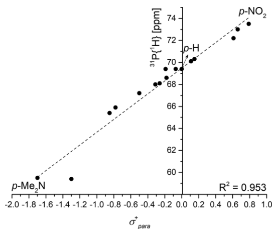
Figure 5. Hammett plot of the \sigma^+_{para} constants against the ^{31}P\{^1H\} chemical shift of azophosphonium salts 1a-p .
