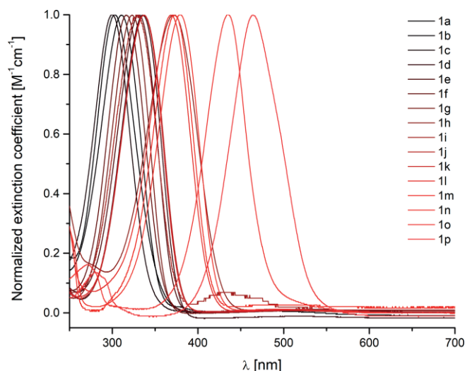
Figure 4. UV/Vis spectra of azophosphonium salts 1a-p .
