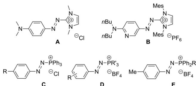
Figure 1. Reported azoimidazolium salts ( A , B ) and azophosphonium salts ( C , D , E ).
