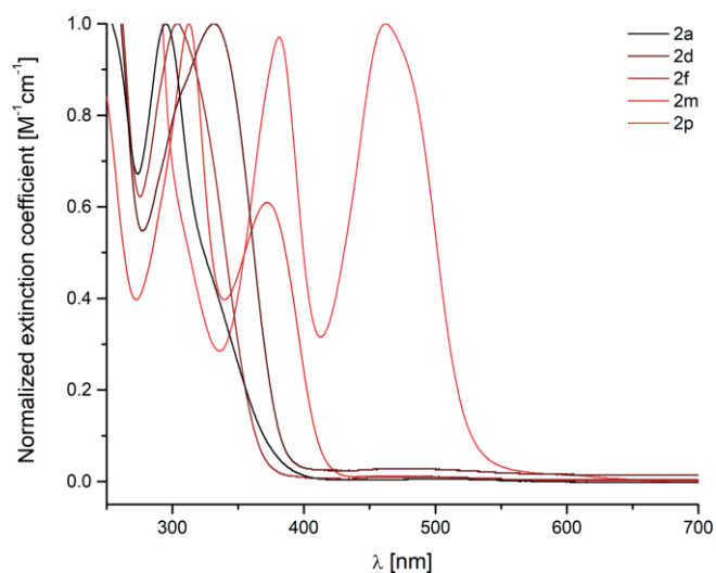
Figure 7. UV/Vis spectra of azophosphonium salts 2a,d,f,m (0.006M in CH 3 CN; 2p in dry DCM).
