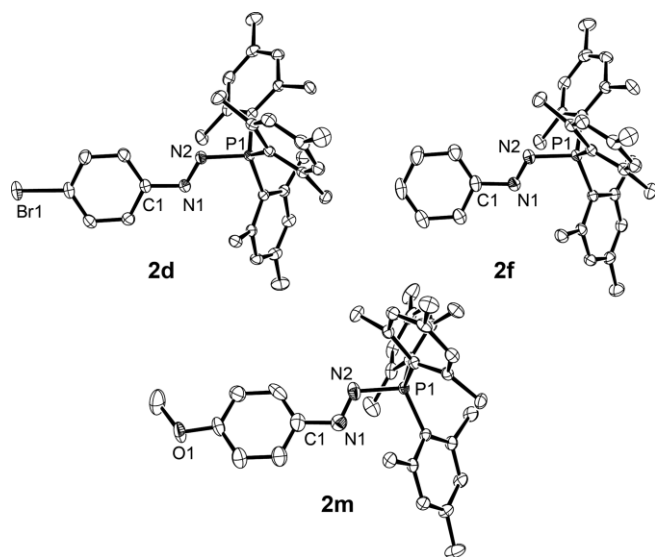
Figure 8. Molecular structures of 2d,f,m [ p -R-(C 6 H 5 )N 2 (PMe 3 )] [BF 4 ] (displacement ellipsoids are set at 30 % probability, hydrogen atoms, disordered solvent molecules and noncoordinating BF 4 anion are omitted for clarity). Selected bond length [Å] and torsion angles [°] for 2d : P1–N2 1.7544(14), N2–N1 1.249(2), N1–C1 1.424(2); P1–N2–N1–C1 –176.60(11). 2f : P1–N2 1.7545(12), N2–N1 1.2437(17), N1–C1 1.4316(19); P1–N2–N1–C1 –178.18(9). 2m : P1–N2 1.736(2), N2–N1 1.214(3), N1–C1 1.432(3); P1–N2–N1–C1 –177.86(17).
