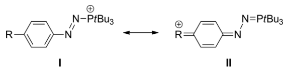
Figure 2. Resonance structures I and II of azophosphonium cations.
