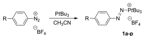
Scheme 1. Synthesis of arylazophosphonium tetrafluoroborates 1 , R = NO 2 ( a ), CN ( b ), CF 3 ( c ), Br ( d ), Cl ( e ), H ( f ), F ( g ), C 6 H 5 ( h ), OC(O)CH 3 ( i ), C(CH 3 ) 3 ( j ), CH 3 ( k ), OC 6 H 5 ( l ), OCH 3 ( m ), OCH(CH 3 ) 2 ( n ), NH 2 ( o ), N(CH 3 ) 2 ( p ).
