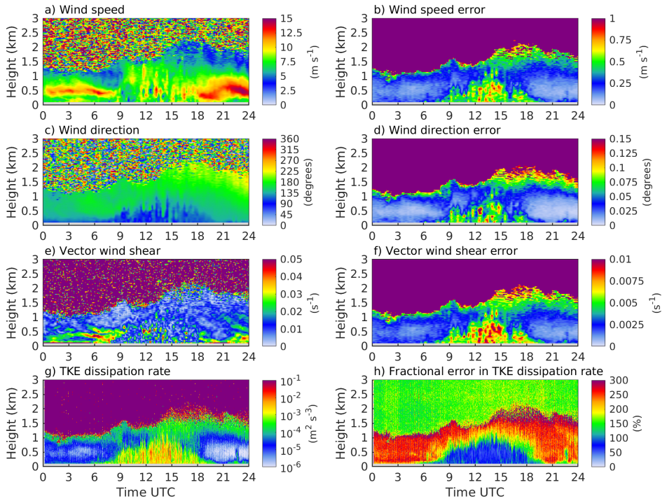
Figure 3: Time–height plots of wind speed (a), wind direction (c), vector wind shear (e), TKE dissipation rate (g), and their respective errors (b,d,f,h) calculated from Halo DL measurements on 31 July 2015 at Jülich, Germany.
