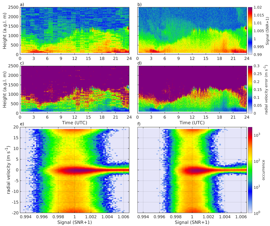
Figure 4: Time–height plots of signal (a–b) and radial velocity uncertainty estimates (c–d), and 2D–histogram plots calculated from radial velocity and signal (e–f) before (a,c,e) and after (b,d,f) the correction of the bias in SNR. Plotted measurement were taken on 5 May 2017 at Hyytiälä, Finland.
