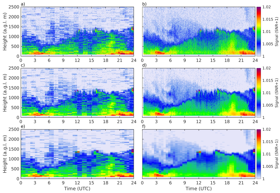
Figure 6: Time–height plots of signal before (a,c,e) and after (b,d,f) the background correction in original temporal resolution (a,b) and averaged to 3 minute (c,d) and to 30 minutes (e,f) temporal resolutions calculated from measurement taken on 5 May 2017 at Hyytiälä, Finland.
