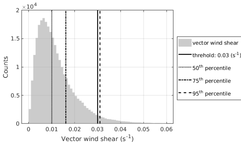
Figure 2: Histogram showing the distribution of vector wind shear values within the ABL and vertical lines depicting a selected threshold value for describing significance vector wind shear (solid), as well as the 50 th (dotted), 75 th (dash-dotted), and 95 th (dashed) percentile values calculated from measurements during July 2015 at Jülich, Germany.
