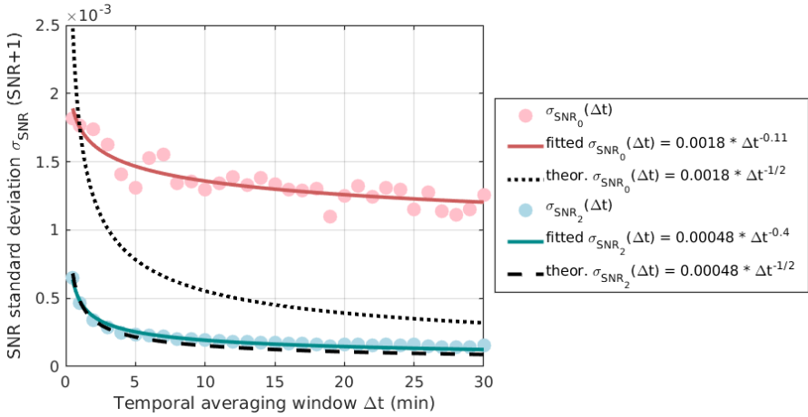
Figure 5: Standard deviation in Halo DL SNR before ( \sigma_{\text{SNR}_0} ) and after ( \sigma_{\text{SNR}_2} ) the background correction (following the notation in Paper II ) calculated from a clear-sky period between two consecutive background checks from 1:00 and 2:00 UTC and data contained in range gates at about 3000m to 9600 m above ground level on 6 July 2015 at Jülich, Germany as a function of window length used in temporal averaging of the SNR ( \Delta t ). The solid lines represent the one-term power series fits ( f(\Delta t) = a * \Delta t^b ) for the \sigma_{\text{SNR}_0} and \sigma_{\text{SNR}_2} , and the dotted and dashed lines represent the theoretical values for the \sigma_{\text{SNR}_0} and \sigma_{\text{SNR}_2} , respectively, when assuming that the \sigma_{\text{SNR}} decreases, i.e. the sensitivity improves, by 1/\sqrt{\Delta t} .
