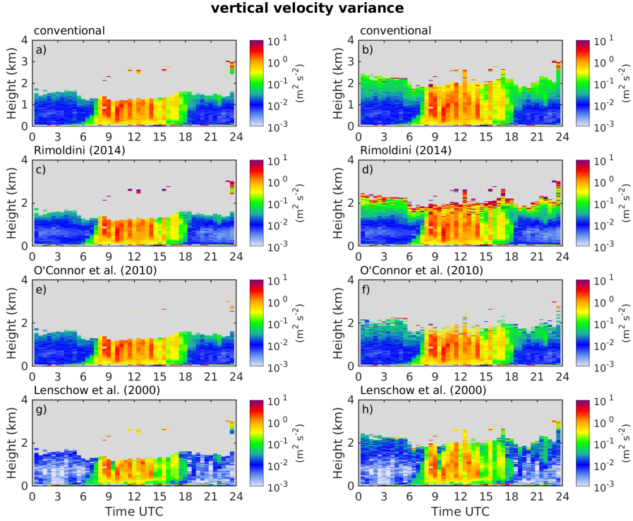
Figure 1: Time–height plots of vertical velocity variance measured with Halo DL on 17 July 2018 at Hyytiälä, Finland calculated by using a conventional method (a,b) and by using three methods presented by Rimoldini (2014), O’Connor et al. (2010), and Lenschow et al. (2000), which provide variance unbiased by noise (c-h). Two SNR thresholds, -23 db (a, c, e, g) and -28 db (b, d, f, h), were used to illustrate their impact on data availability and highlight the differences in the performance of the methods at the top of the ABL where the SNR is generally low.
