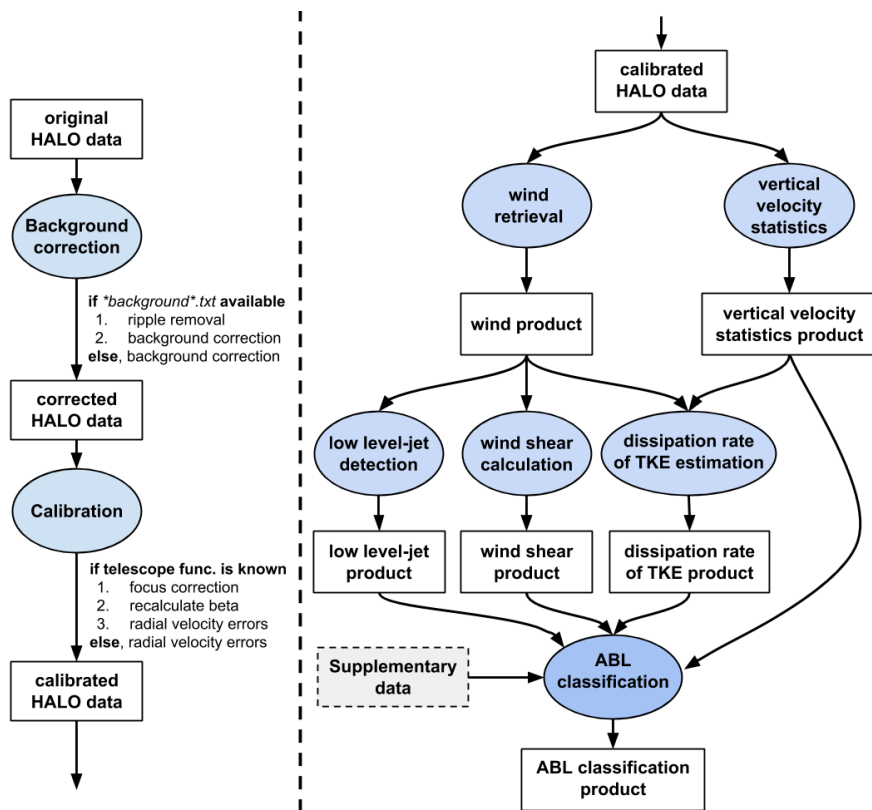
Figure 7: Sketch diagram of the Halo lidar toolbox processing chain illustrating the data processing steps from the original uncorrected data to the ABL classification product.
