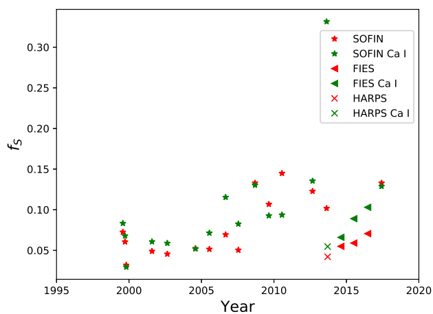
Fig. 4. Spot filling factors calculated with combined lines, compared to those where only the Ca I line was used. SOFIN, FIES, and HARPS observations are distinguished from each other.
