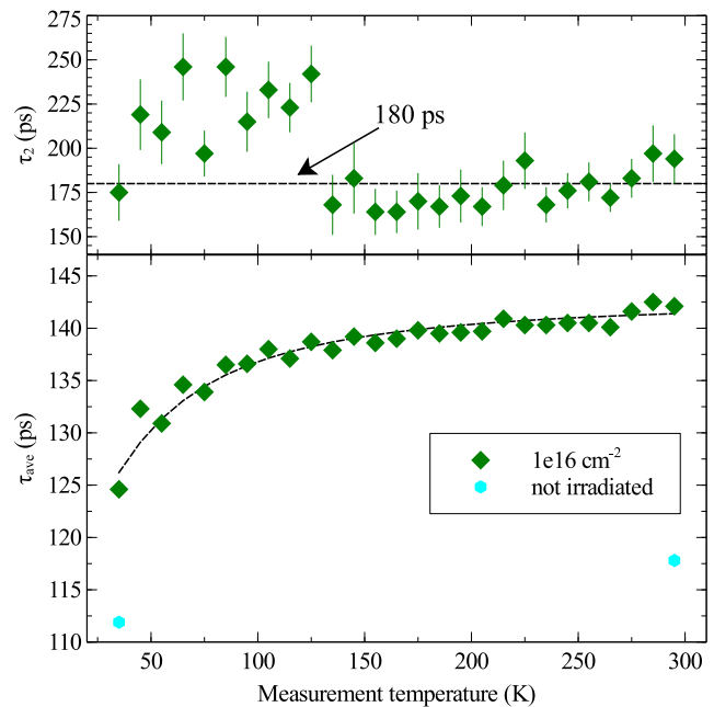
FIG. 2. Temperature behavior of the average positron lifetime \tau_{ave} in the irradiated sample after annealing at RT. The upper panel shows the second lifetime component \tau_2 . The temperature behavior of these data suggests that structural defects such as dislocations and grain boundaries compete with vacancy defects in positron trapping at low temperatures. The solid curve shows the best fit of the two-defect model described in the text.
