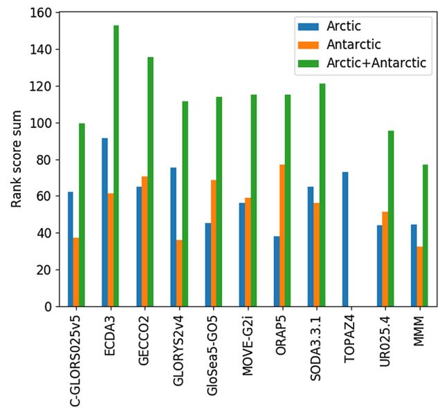
Fig. 26 Sums of rank scores of various diagnostic variables for individual ORAs and their mean product (MMM). The ranking is based on standard deviations of differences between the ORAs and observational data in the Arctic (blue bars), Antarctic (orange bars) and both added together (green bars) shown in Table 3. A smaller sum indicates a closer agreement with the observational data and a better performance. The Arctic snow depth and net liquid ocean heat transport diagnostic rank scores were excluded from the sums as GECCO2 did not provide snow depth and the ocean transport diagnostic provided the mean values of net transports only
