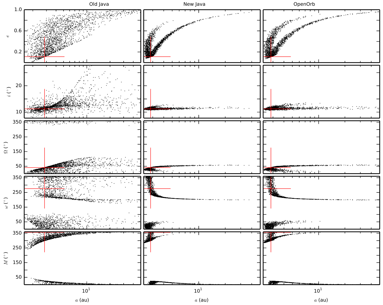
Fig. 9. Same as Fig. 4 but for asteroid (274721) 2008 UH 155 with twelve transits.
