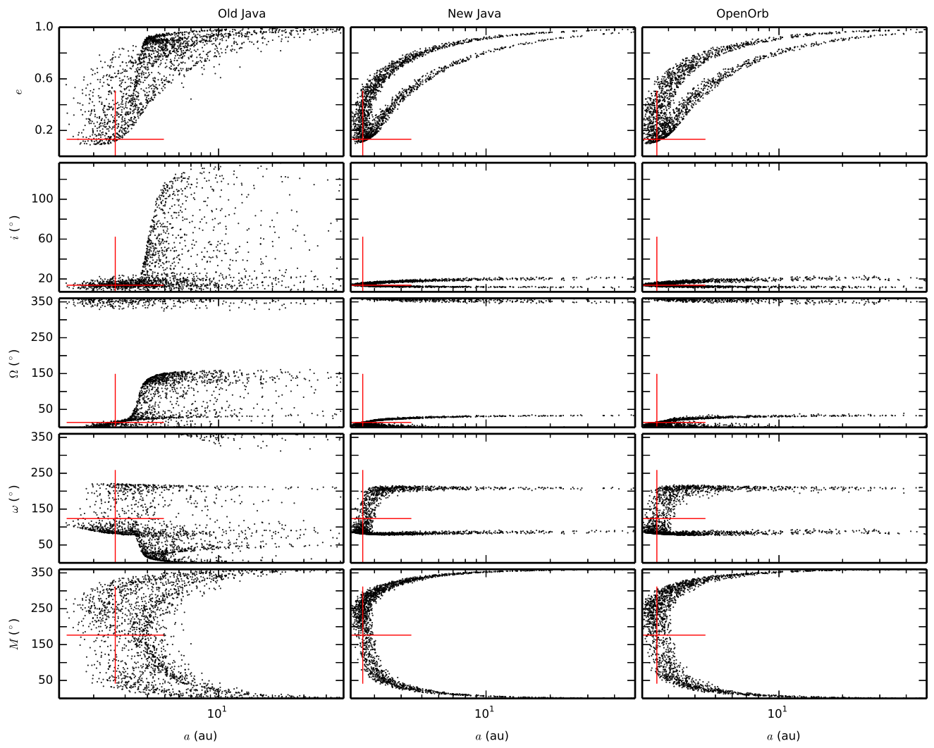
Fig. 8. Same as Fig. 4 but for asteroid (150016) 2005 UB 353 with nine transits.
