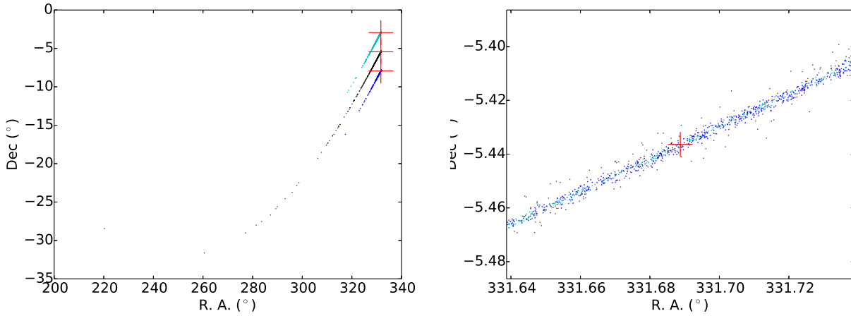
Fig. 2. Left: Spread on the sky after two days of propagation for an object with three transits. Black points represent the spreading of the orbits according to the old data model, blue points according to the new data model, turquoise points are validation points from OpenOrb, and the red cross is the correct position according to JPL Horizons. The points for the new data model and validation are shifted in declination for illustration purposes. Right: The magnification of spread across the line of variation. The width of the spread is around 20'' .
