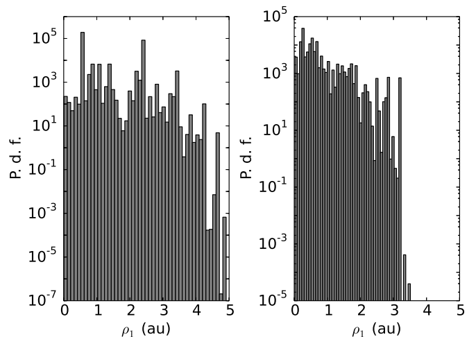
Fig. 11. Comparison of marginal pdfs in the proposed ranges of orbits for an asteroid with three transits in the old independent observation model ( left ), and the new normal-point model ( right ).
