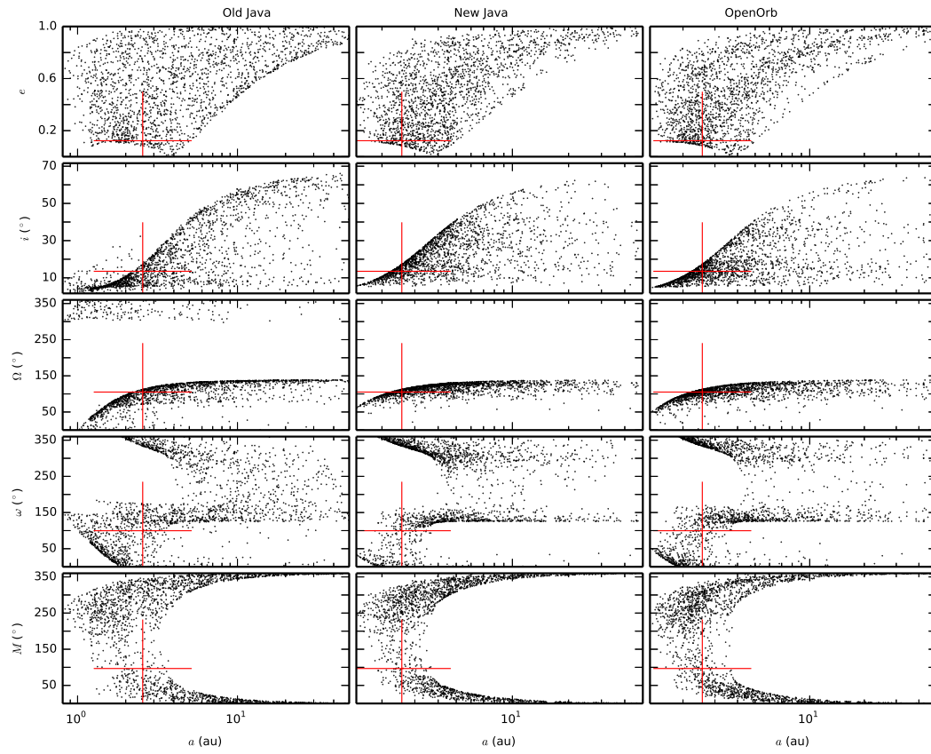
Fig. 5. Same as Fig. 4 but for asteroid (414265) 2008 GC 113 , with four transits.
