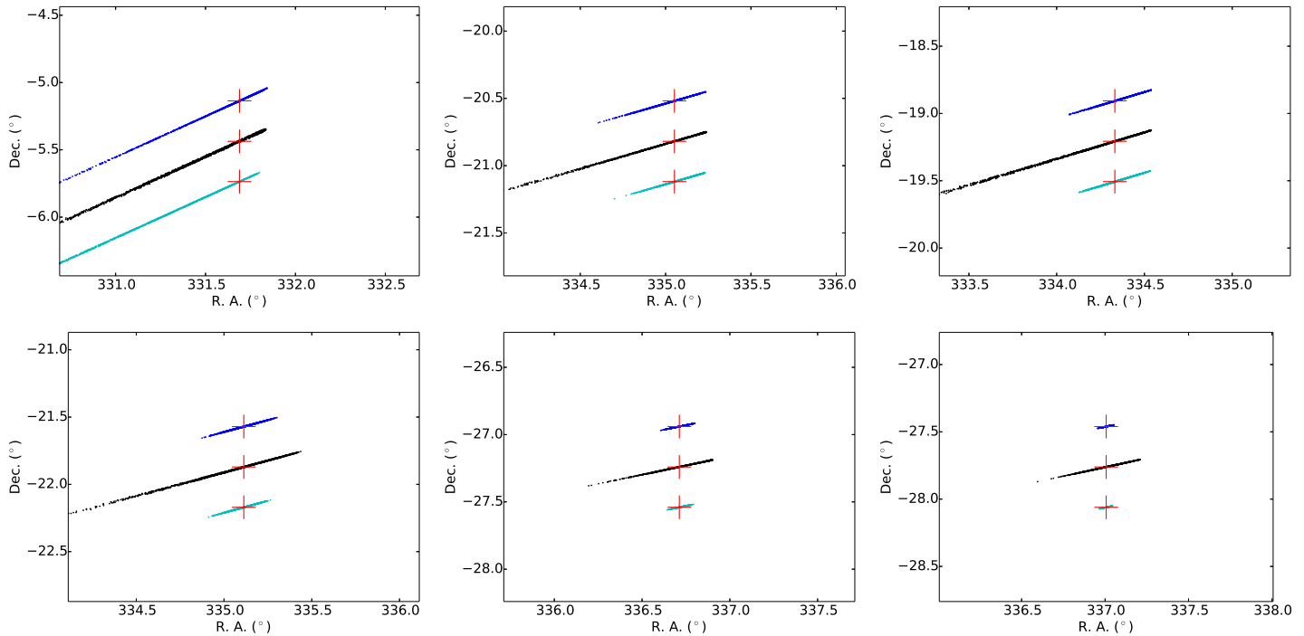
Fig. 3. Comparison of the distribution of sky positions after two days of propagation for asteroids with a different number of transits (From left to right and from top to bottom: 3, 4, 5, 6, 9, 12). The scale is the same for all cases. Black points represent the spreading of the orbits according to the old data model, blue points according to the new data model, turquoise points are validation points from OpenOrb, and the red cross is the correct position according to JPL Horizons. The points for the new data model and validation are shifted in declination for illustration purposes. For the three-transit case, the real spread along the line of variation does not fit on the same scale with other cases. The spread is in the order of 15^\circ for the new data model and 60^\circ for the old data model (Fig. 2 left).
