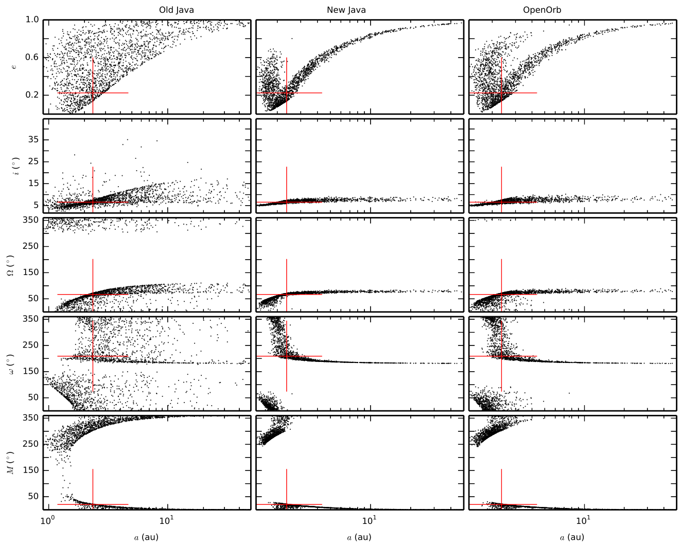
Fig. 7. Same as Fig. 4 but for asteroid (420834) 2013 JX 10 with six transits.
