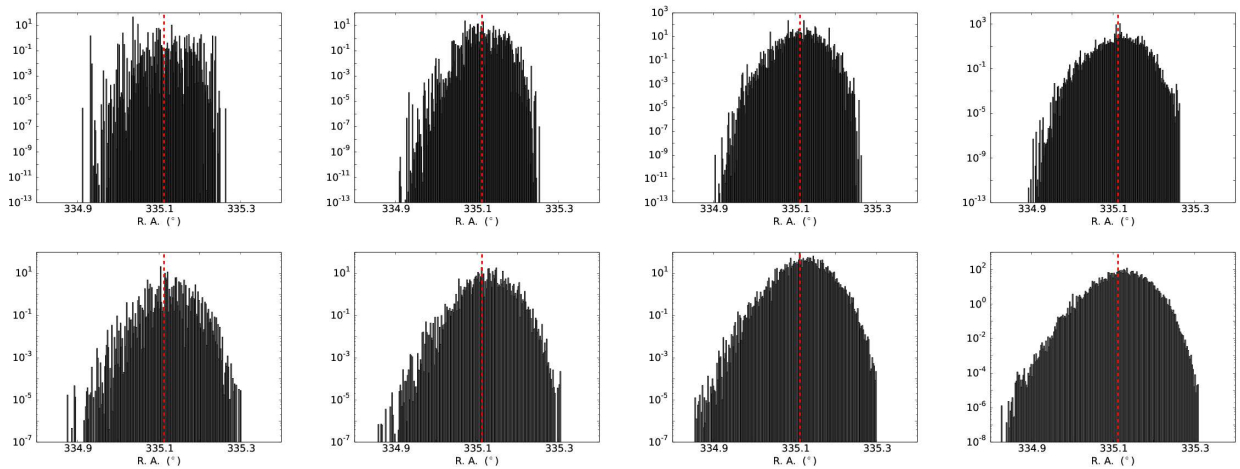
Fig. 10. Comparison of the sample orbit sizes and their respective weights between two codes (Java, top; OpenOrb; bottom) as a function of the right ascension of the sky positions of the propagated orbits for (420834) 2013 JX 10 , meaning an object with six transits. The sample sizes in each column from left to right are 2 000, 5 000, 20 000, and 50 000 orbits respectively. The correct position is designated by a vertical red dashed line in each case.
