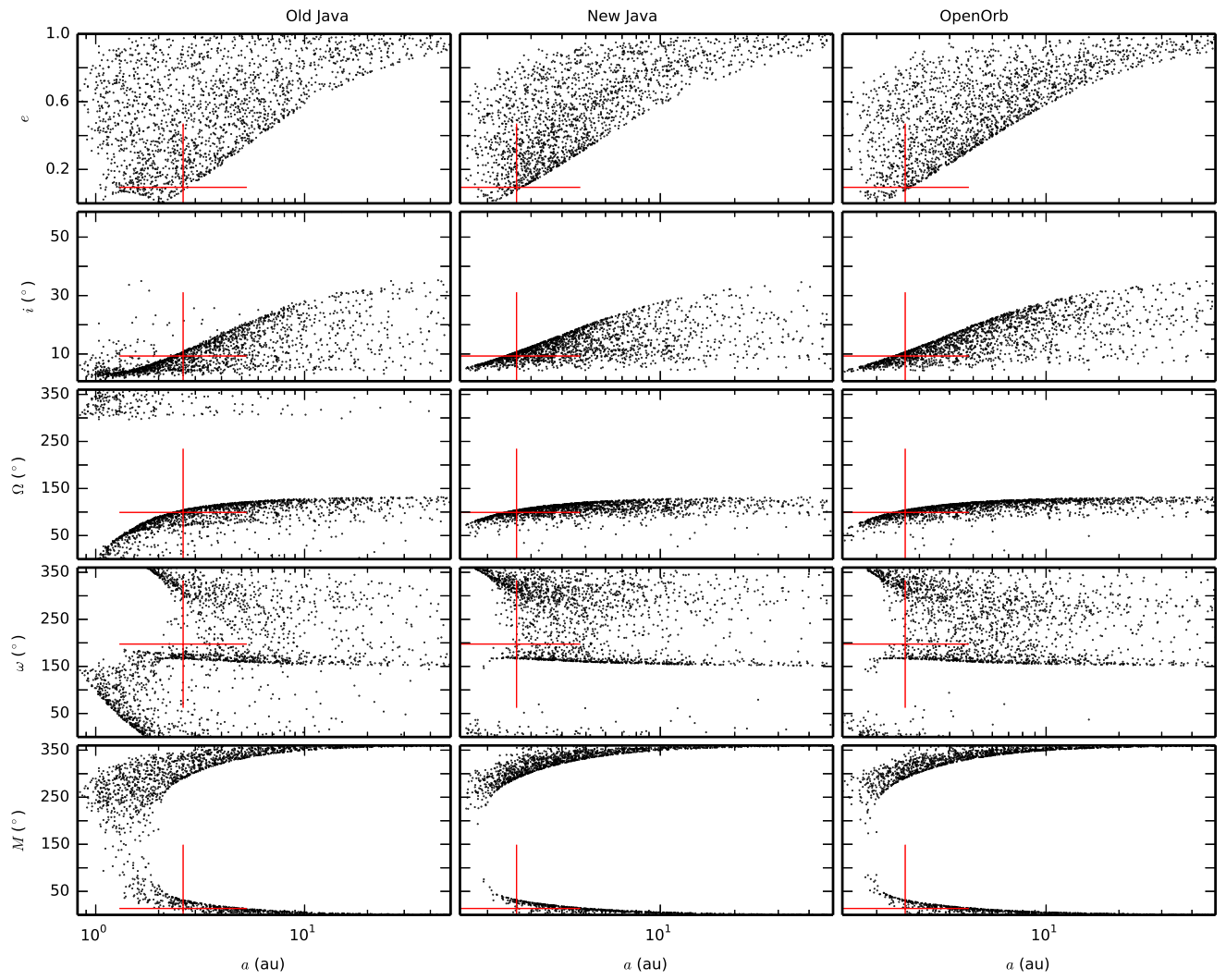
Fig. 6. Same as Fig. 4 but for asteroid (462915) 2011 AC 21 with five transits.
