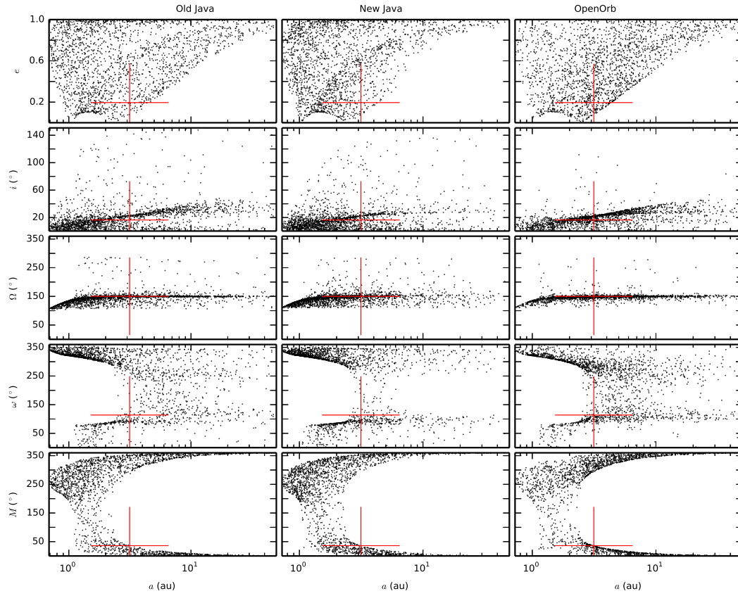
Fig. 4. Asteroid (425387) 2010 CZ 61 , with three transits. Comparison of Keplerian elements as a result of orbital inversion with different methods and codes. Left column from top to bottom: Keplerian elements e , i , \Omega , \omega and M as a function of a . Middle column: same elements, but for Java code with normal-point treatment. Right column: OpenOrb with normal-point treatment. The red cross denotes the correct position of the object.
