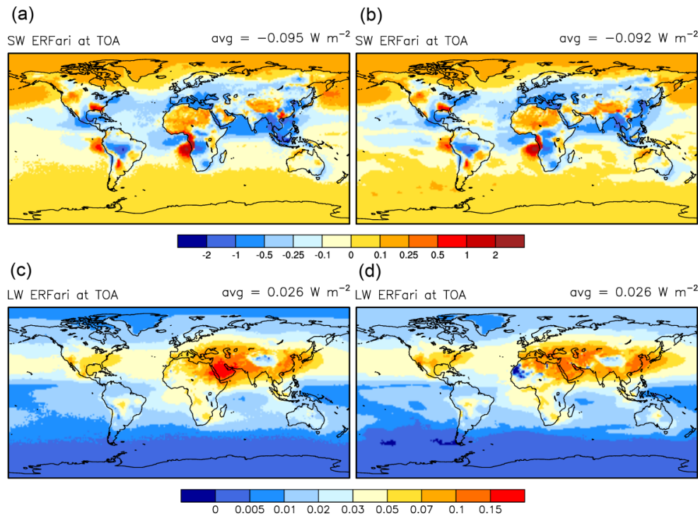
Figure 9. Shortwave (SW, a and b ) and longwave (LW, c and d ) ERF at the top of the atmosphere (TOA) for the simulations NUDGE_PD–NUDGE_PI ( a and c ) and AMIP_PD–AMIP_PI ( b and d ). Note the different color scales. Note also that the semi-direct effect is not included here, since ERFari in this study corresponds to the “direct radiative forcing” component in Ghan (2013).
