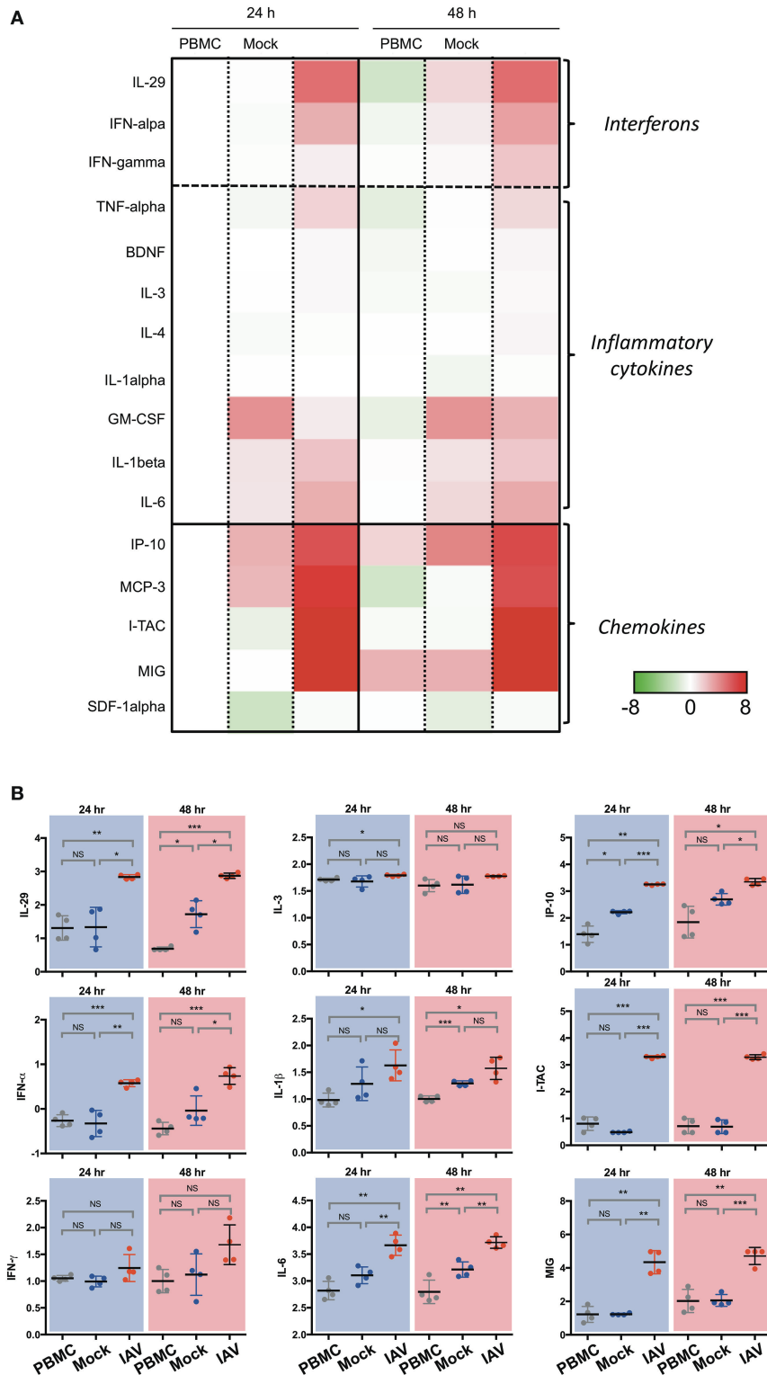
FIGURE 2 | Luminex analysis of culture supernatants of PBMC, Mock, and IAV infection at 24 and 48 h. (A) Heatmap of interferon, selected cytokines and chemokines. The colors indicate the relative change (log 2 fold change) of average analyte concentration in supernatant of PBMC, Mock, and IAV infection at 24 and 48 h compared to PBMC at 24 h. For each analyte, the relative concentration is shown as a scale from 8 and -8. (B) Statistically significantly upregulated cytokine and chemokine concentrations measured by Luminex multiplex assay on a custom 23-plex plate. Cytokines and chemokines are reported in log 10 pg/ml. PBMC, peripheral blood mononuclear cell only sample; Mock, co-culture sample without H3N2-infection of nasal epithelium; IAV, co-culture of H3N2-infected nasal epithelium. All data represent the mean \pm SD. *** P < 0.001; ** P < 0.01; * P < 0.05; NS, not significant.
