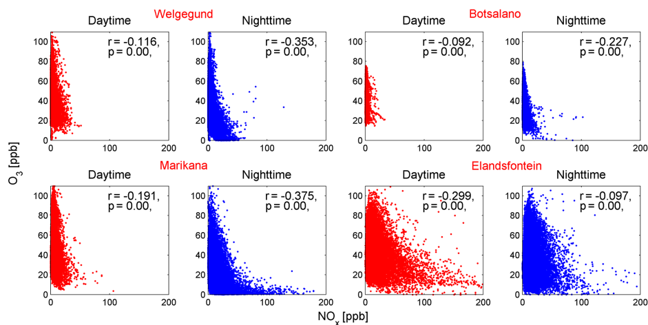
Figure A6. Scatter plots of \text{O}_3 vs. \text{NO}_x for daytime (09:00 to 16:52 LT), and night-time (17:00 to 08:52 LT) at Welgegend, Botsalano, Marikana, and Elandsfontein. The correlation coefficient ( r ) has a significance level of p < 10^{-10} , which means that r is statistically significant ( p < 0.01 ).
