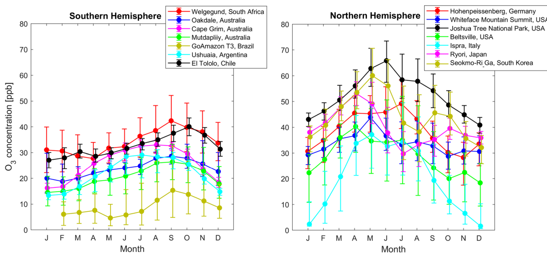
Figure 4. Seasonal cycle of O_3 at rural sites in other parts of the world. The dots indicate monthly median (50th percentile) and the upper and lower limits the 25th and 75th percentiles, respectively, for monthly O_3 concentrations. The data are averaged from May 2010 to December 2014, except in a few instances in which 2014 data were not available.
