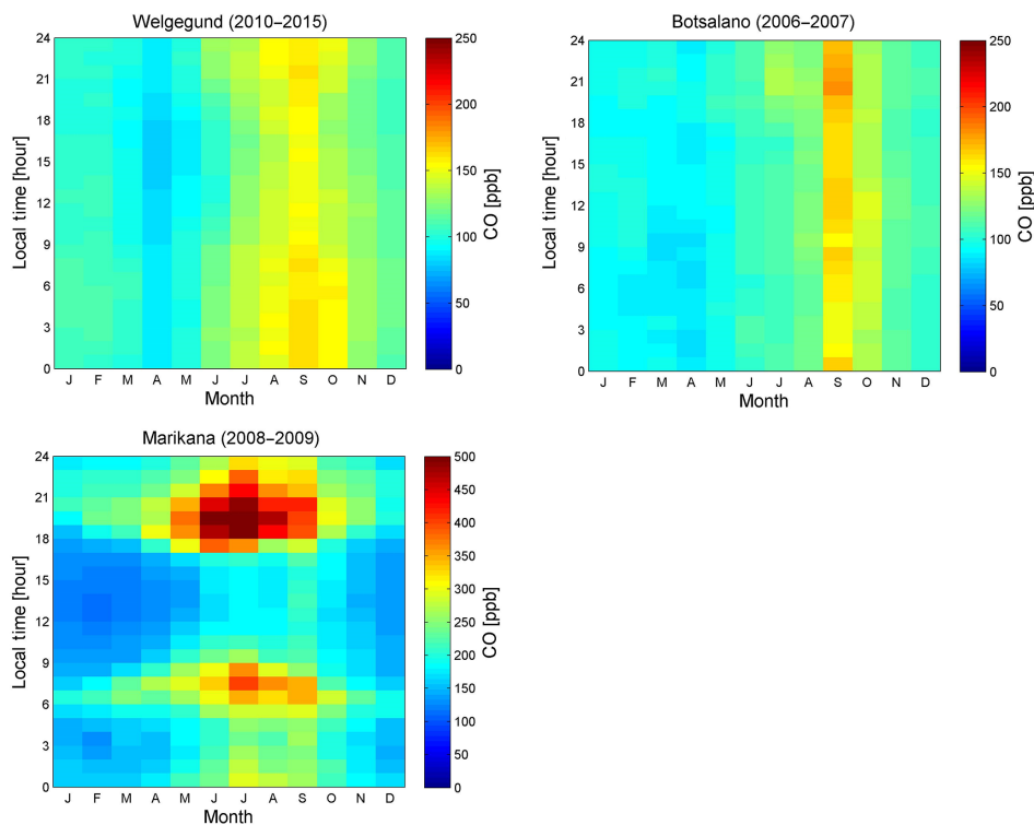
Figure A5. Seasonal and diurnal variation in CO at Welgegend, Botsalano, and Marikana (median values of CO concentration were used). Note that CO was not measured at Elandsfontein.
