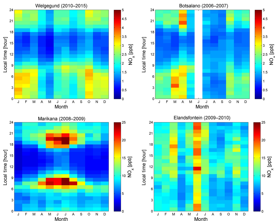
Figure A4. Seasonal and diurnal variation in \text{NO}_x at Welgegend, Botsalano, Marikana, and Elandsfontein (median values of \text{NO}_x concentration were used).
