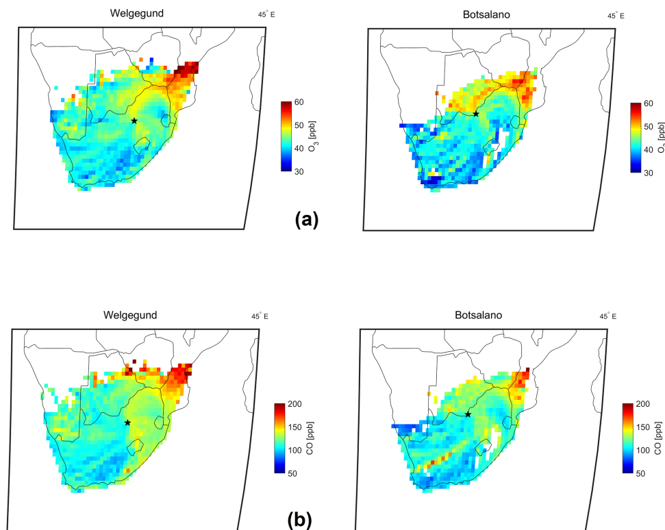
Figure 5. Source area maps of (a) \text{O}_3 concentrations and (b) CO concentrations for the background sites Welgegund and Botsalano. The black star represents the measurement site and the colour of each pixel represents the mean concentration of the respective gas species. At least 10 observations per pixel are required.
