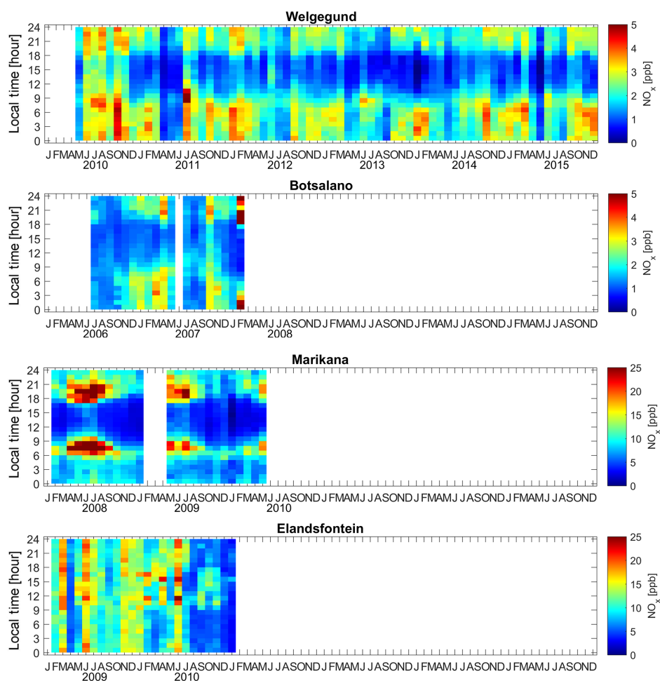
Figure A7. Time series of monthly median \text{NO}_x concentrations for each hour of the day at the four sites.
