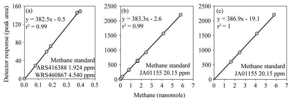
Figure 3. FID response to methane fitted with a linear regression calibration. The inclusion (a, b) or exclusion (c) of low methane values causes the calibration slope and intercept to vary. However, the observed variation in the calibration slope does not have a significant effect on the final calculated concentrations of methane. In contrast, variation in the intercept does have an effect on the final concentrations of methane.
