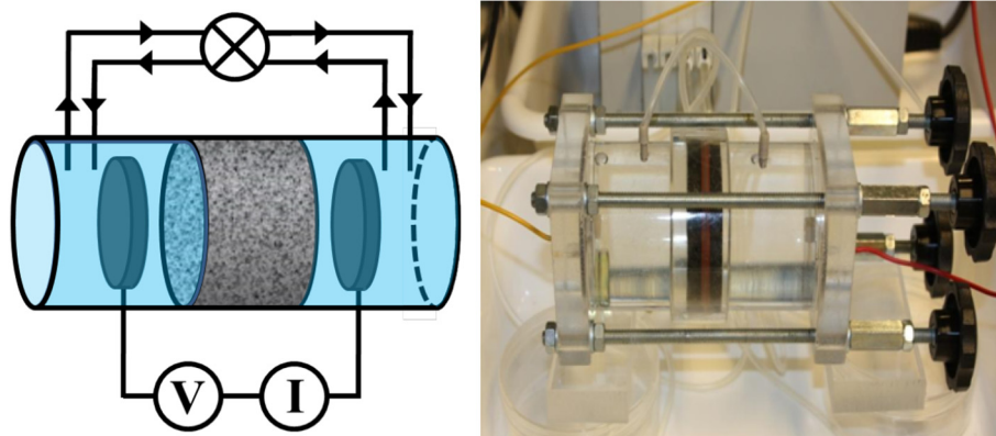
Fig. 2. A schematic diagram of the electromigration equipment (left) that consists a voltage source and meter (V), ammeter (I), peristaltic pump (X), platinum electrodes and drill core sample and a photograph of the electromigration experimental vessel (right) showing the drill core samples in the middle of two chambers.
