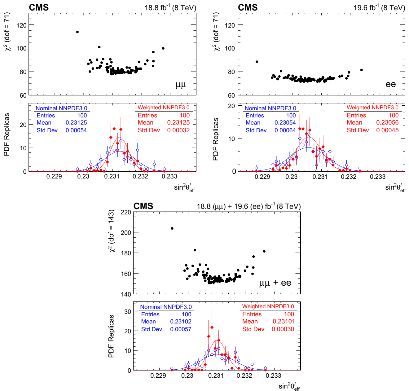
Fig. 6 The upper panel in each figure shows a scatter plot in \chi_{\text{min}}^2 vs. the best-fit \sin^2 \theta_{\text{eff}}^{\ell} , for 100 NNPDF replicas in the muon channel (upper left), electron channel (upper right), and their combination (below). The
