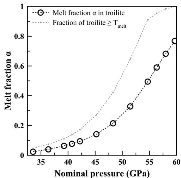
Fig. 11. Profile of troilite melting over nominal pressures in model no. 2. The blank circles are the melt fractions \alpha for the bulk material. The greyed line represents the fraction of material that reaches melting temperature.
