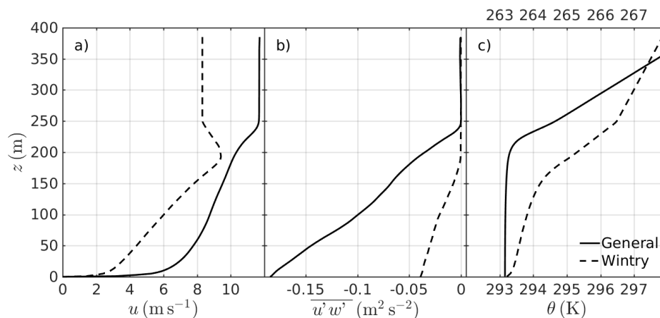
Figure 6. The vertical profile of (a) streamwise velocity u ( \text{m s}^{-1} ), (b) Reynolds stress \overline{u'w'} ( \text{m}^2 \text{s}^{-2} ), and (c) potential temperature \theta (K) at the inflow boundary for the general (solid line) and wintry (dashed line) inflow conditions. The top x -axis for \theta is for the wintry conditions.
