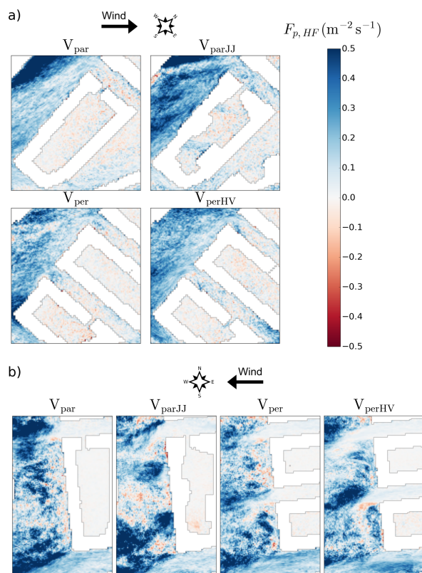
Figure A2. 5-min mean high-frequency vertical turbulent particle flux density F_{p,HF} ( m^{-2} s^{-1} ) at z = 20 m under the (a) general and (b) wintry inflow conditions. The analysis area is marked in Figure 2 with a black solid line.
