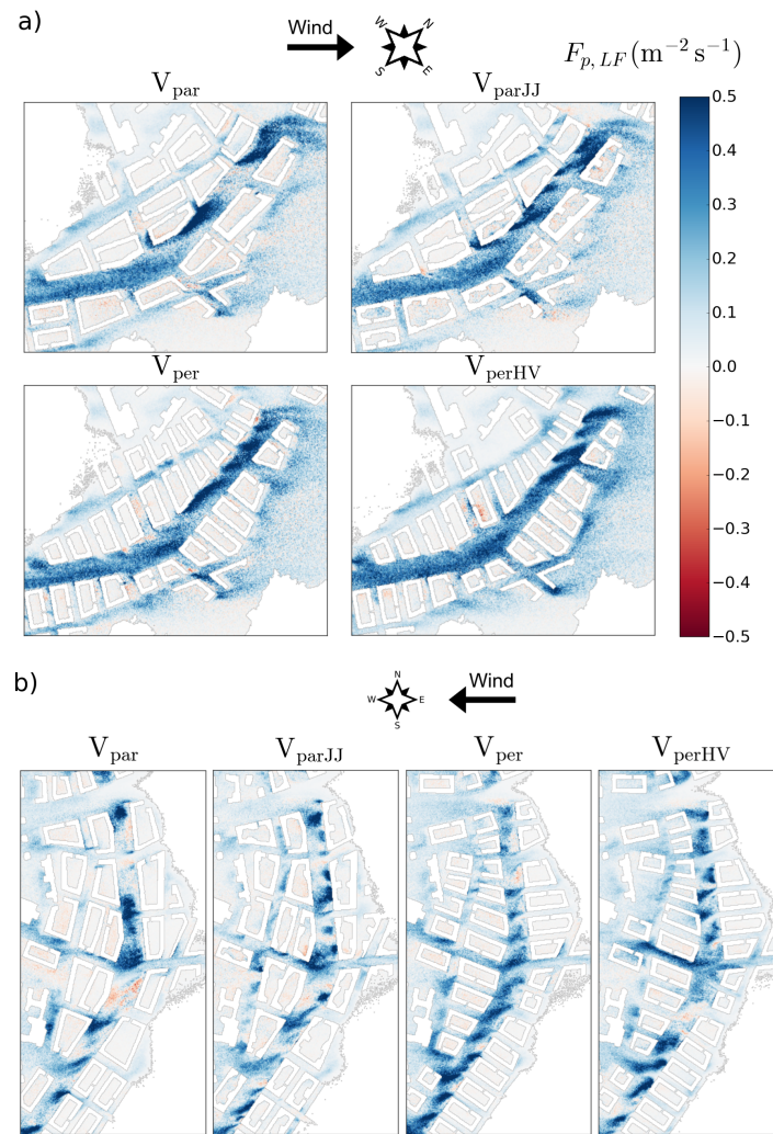
Figure 11. 40-min mean low-frequency vertical turbulent particle flux density F_{p,LF} ( m^{-2}s^{-1} ) at z = 20 m under the (a) general and (b) wintry inflow conditions. Positive values indicate upward flux.
