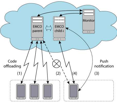
Fig. 6: Multi-tenancy and horizontal scaling in EMCO.
