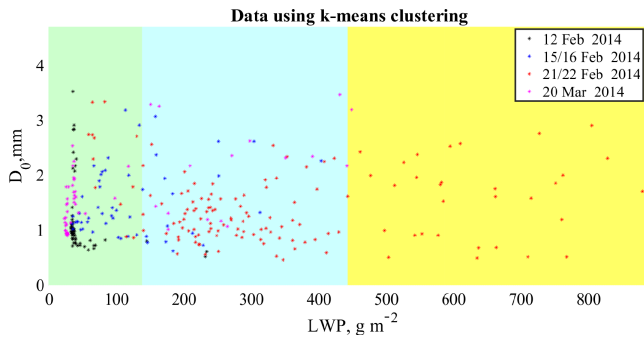
Figure 3. Plot of median diameter D_0 with respect to LWP for the three cluster regions, LR, MR and HR, (green, cyan, yellow) obtained on four snowfall days of BAEC IOP campaign. Black, blue, red and magenta points respectively represent the data for 12, 15/16, 21/22 February and 20 March 2014. The k -means clustering highlights the weak dependence of the classes from D_0 .
