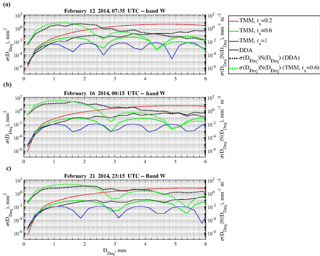
Figure 12. Horizontally polarized cross section \sigma , expressed as a function of the diameter disk-equivalent D_{Deq} at W band by comparing DDA computations (black line) and TMM computations (red, green and blue lines, matching r_s = 0.2 , r_s = 0.6 and r_s = 1 ). The product between \sigma and PIP-derived snowflake size distribution N shows the main contribution of particle size in terms of diameter disk-equivalent for DDA computations (dotted black line) and TMM computations ( r_s = 0.6 , dotted green line).
