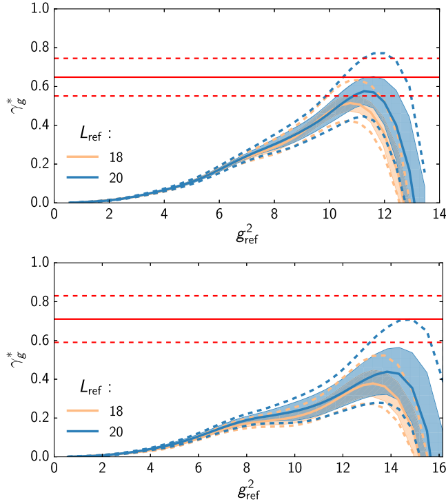
FIG. 7. Fit to function (9) for all couplings g_{GF}^2(\beta_L, L_{ref}) with the chosen set of discretizations: (top) at c_t = 0.3 and (bottom) at c_t = 0.35 . The shaded bands indicate the statistical errors for g_{ref}^2 being the measured value, and dashed lines indicate how the result changes when g_{ref}^2 is varied within its statistical errors.
