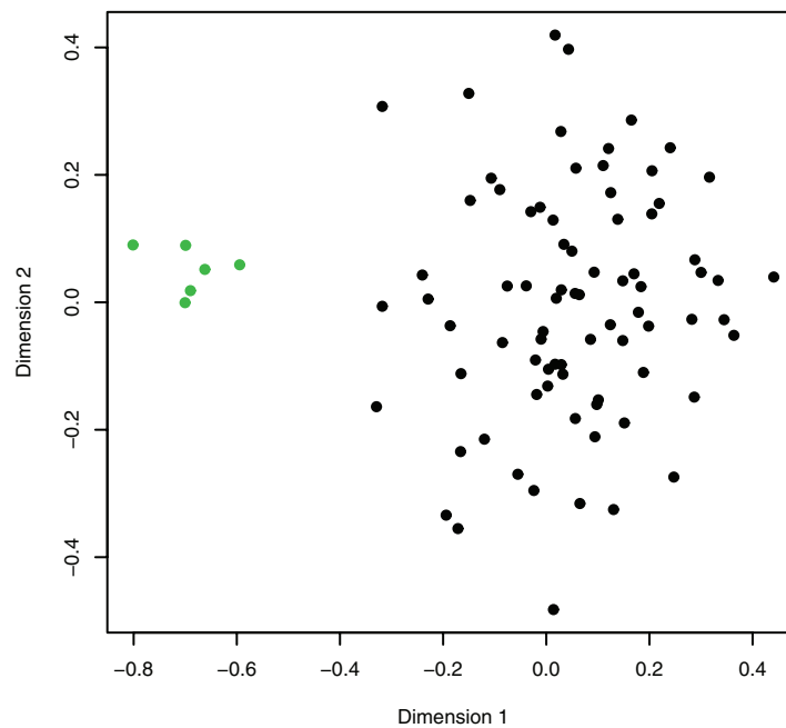
Figure 3. Genome wide expression profiles in normal colon mucosa. An MDS plot created with the 100 most differentially expressed genes between CRC (green) mice and mice without cancer (black). The expression profiles of the six mice which developed carcinoma up to 18 months of age form a distinct cluster in the plot.
