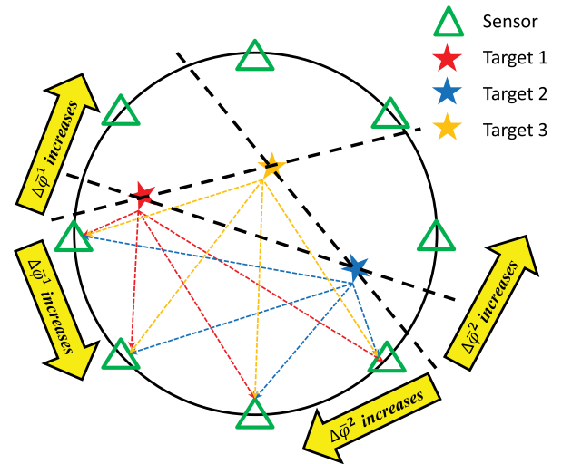
FIGURE 8. Sensor separation for 2D three-target detection.
