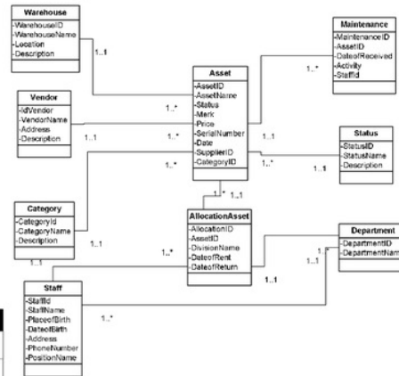
Figure 3. Class Diagram Of Asset Management System
