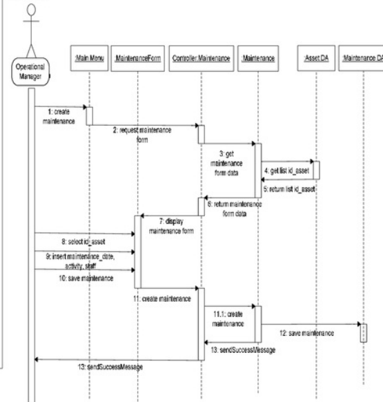
Figure 4. Sequence Diagram Of Asset Maintenance
