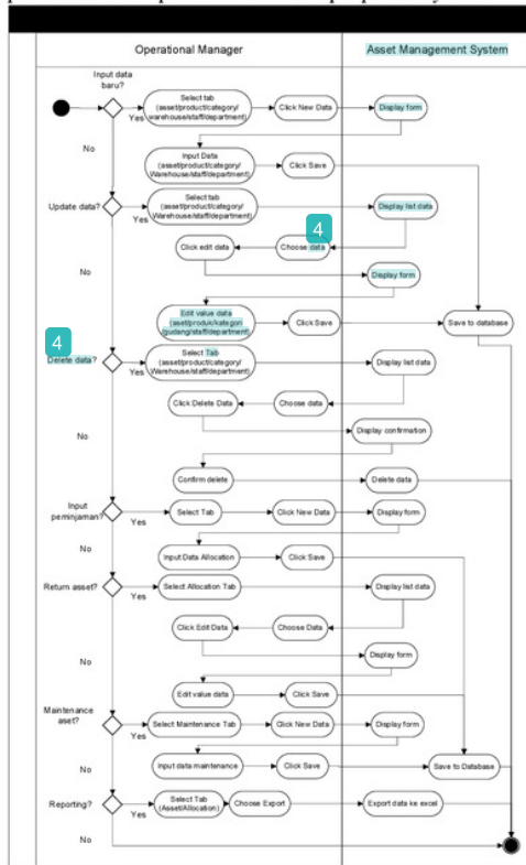
Figure 2. Activity Diagram Of Asset Management System
