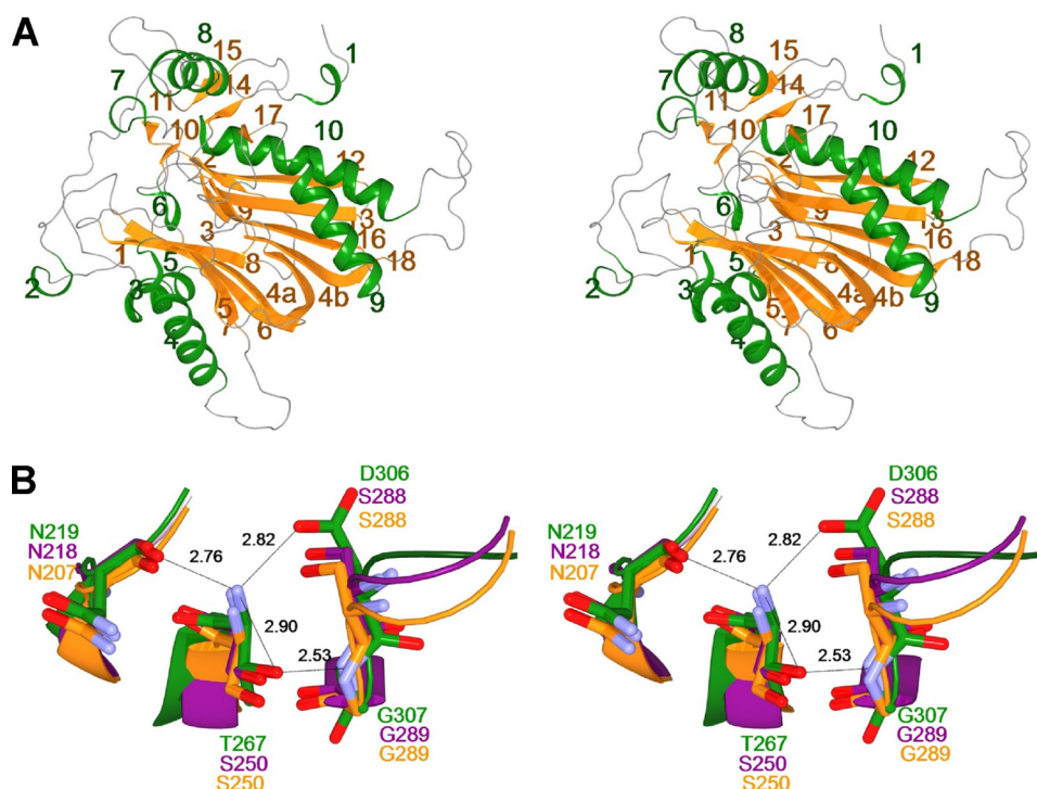
FIGURE 2. Stereo view of subunit structure and catalytic center of NylC A . A , the overall structure of the heterodimer (molecule A) is shown as a ribbon diagram. Ten helices (H1–H10) and eighteen \beta -strands (S1–S18) are colored in green and orange, respectively. H1–H6 and H8–H10 are \alpha -helices. H7 is a 3_{10} helix. B , the structure around the catalytic residue Thr-267 of NylC A (green) is superimposed onto the structure of DmpA (PDB ID code, 1B65; magenta) and BapA (PDB ID code, 3N33; orange). Possible hydrogen bonds in NylC A are indicated as dotted lines with the distances listed in angstroms.
