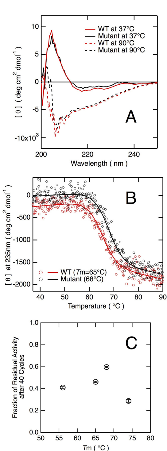
FIGURE 8. Effects of mutations of anti-hCG VHH on its biophysical characteristics. A, CD spectra of wild-type and N52S/N74S/N84T VHH (25 \mu\text{M} ) at 37 and 90 °C in HBS-EP buffer without EDTA. B, equilibrium thermal unfolding curves of wild-type and N52S/N74S/N84T VHH were measured by changes in ellipticity at 235 nm at a protein concentration of 25 \mu\text{M} . Curves fitted by standard thermodynamic equations (63) are presented as solid lines, and T_m values of wild-type VHH and N52S/N74S/N84T mutant VHH were estimated to be 65 and 68 °C, respectively. C, T_m values and residual activities of wild-type VHH and VHH mutants (100 nm) after 40 heating-cooling cycles. The T_m values of disulfide mutants C22W/A49C/I70C/C96A (56 °C) and A49C/I70C (74 °C) are from Hagihara et al. (33). Wild-type and N52S/N74S/N84T mutant anti-hCG VHH are abbreviated as WT and Mutant, respectively. Error bars represent S.D. deg, degrees.
