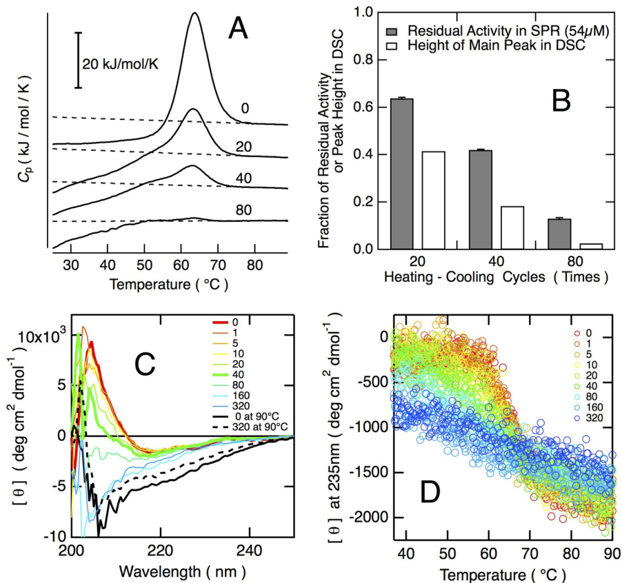
FIGURE 10. Comparison of heat-induced structural changes and denaturation of anti-hCG VHH. A , VHH heat absorption curves. VHH samples (54 \mu\text{M} in HBS-EP buffer) were subjected to cycles of unfolding at 90 ^{\circ}\text{C} for 5 min and refolding at 20 ^{\circ}\text{C} for 5 min in a thermal cycler. The broken lines represent the extrapolated linear baseline of the unfolded state. The number of cycles is indicated on each curve. B , comparison between residual activities measured by SPR and the main peak of heat absorption curves corresponding to intact VHH after heat treatment. The main peaks were estimated by subtracting the baseline (unfolded state) from the peak heights for all samples, and the resulting heat-treated peak was then divided by the untreated sample peak. Error bars represent S.D. C , CD spectra of heat-treated VHH at 37 ^{\circ}\text{C} in HBS-EP buffer without EDTA. Samples at a protein concentration of 25 \mu\text{M} were subjected to cycles of unfolding at 90 ^{\circ}\text{C} for 5 min and refolding at 20 ^{\circ}\text{C} for 5 min. For comparison, CD spectra of thermally unfolded intact and heat-denatured VHH at 90 ^{\circ}\text{C} are also shown. D , equilibrium thermal unfolding curves of heat-treated VHH measured by changes in ellipticity at 235 nm. Samples were the same as in C . deg , degrees.
