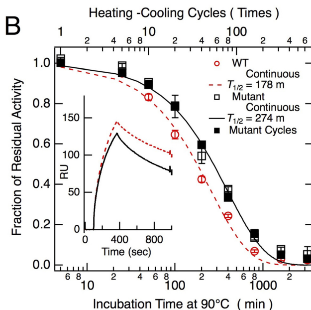
FIGURE 7. Effects of replacement of Asn residues in anti-hCG VHH. A , Asn residues 52, 74, and 84 in anti-hCG VHH-H14 were substituted by Ser, Ser, and Thr, respectively, resulting in the N52S/N74S/N84T mutant. B , N52S/N74S/N84T mutant (100 nm) was treated with heating (90 °C for 5 min)-cooling (20 °C for 5 min) cycles (black closed box) or continuous incubation at 90 °C followed by recooling at 20 °C for 5 min (black open box). The theoretical curve for N52S/N74S/N84T (solid line) was fitted using 0.0025 \text{ min}^{-1} as a first-order kinetic constant k_{\text{den}} . From this k_{\text{den}} , the half-life of the N52S/N74S/N84T mutant was calculated to be 274 min ( m ). Data for wild-type VHH treated with continuous incubation and its theoretical curve are presented as red circles and broken line, respectively. The SPR signals for untreated wild-type (red broken line) and N52S/N74S/N84T (black solid line) VHHs (100 nm) are presented in the inset. In all panels, wild-type and N52S/N74S/N84T mutant VHHs are abbreviated as WT and Mutant, respectively. Error bars represent S.D. CDR, complementarity determining region.
