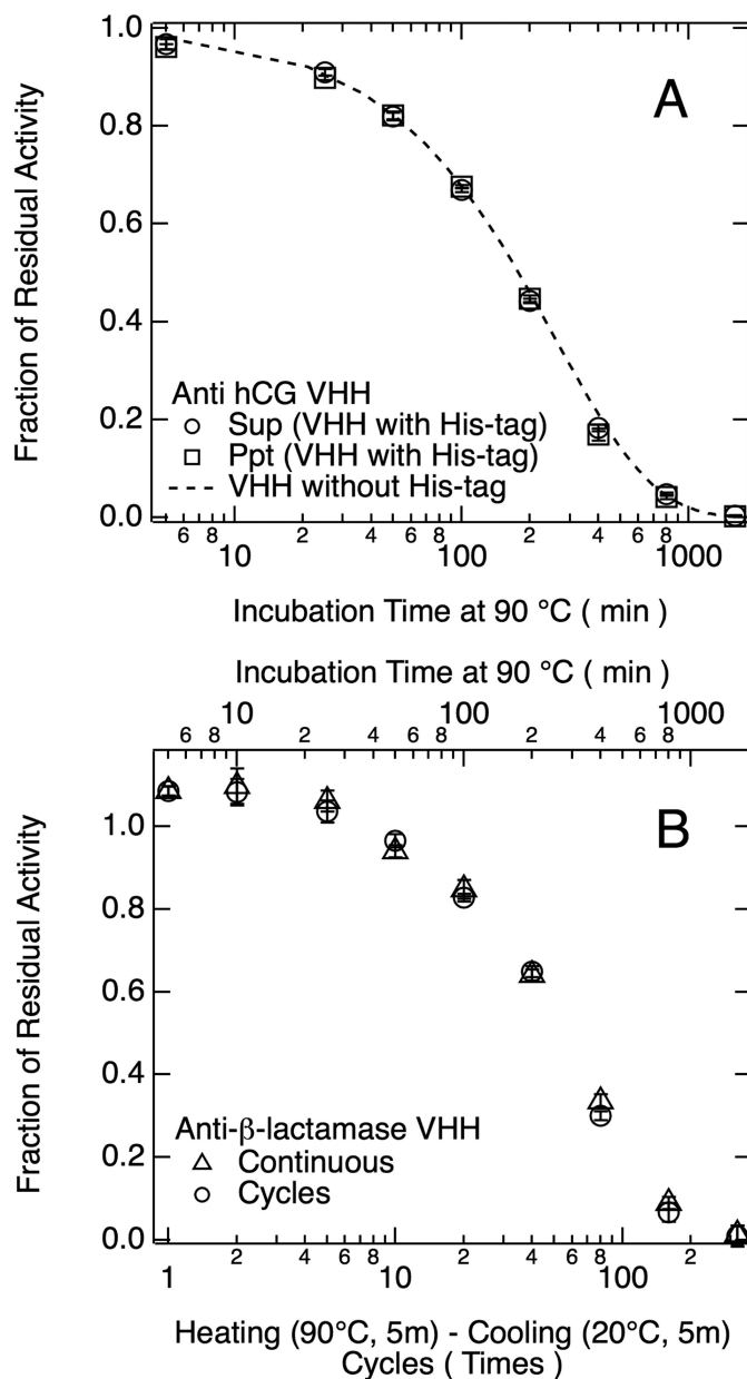
FIGURE 3. Heat resistance of anti-hCG VHH with different preparations and anti- \beta -lactamase VHH. A, anti-hCG VHH samples prepared from E. coli soluble ( circles ) and insoluble ( squares ) fractions were subjected to continuous incubation at 90 °C. Both samples were histidine-tagged at their C termini. B, anti- \beta -lactamase VHH was subjected to heating-cooling cycles ( circles ) or continuous incubation at 90 °C ( triangles ). In heating-cooling cycles, a given number of reaction segments, which consisted of heating at 90 °C for 5 min ( m ) and cooling at 20 °C for 5 min, were repeated. Both experiments were carried out at pH 7.4 in HBS-EP buffer at a protein concentration of 1.3 \mu\text{g}/\text{ml} . Error bars represent S.D. Sup , supernatant; Ppt , precipitate.
