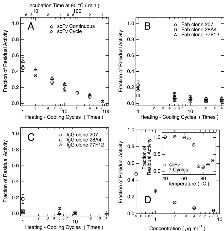
FIGURE 11. Heat-induced irreversible denaturation of anti-hCG antibody fragments. A–C, scFv (A), Fab (B), and IgG (C) samples ( 1 \mu\text{g/ml} ) were subjected to heating ( 90^\circ\text{C} for 5 min)-cooling ( 20^\circ\text{C} for 5 min) cycles at pH 7.4. In addition, dependence of scFv denaturation on incubation time at 90^\circ\text{C} is also shown (A). Residual activity at 20^\circ\text{C} was estimated using the strength of the SPR signal compared with that of SPR signals from a series of diluted untreated samples and is presented as the fraction of the corresponding untreated diluted sample. D, concentration-dependent denaturation of scFv was examined. ScFv samples with the given concentrations were subjected to five cycles of unfolding at 90^\circ\text{C} for 5 min and refolding at 20^\circ\text{C} for 5 min. Inset, scFv ( 1 \mu\text{g/ml} ) was subjected to seven heating-cooling cycles where the heating temperatures ranged from 40 to 90^\circ\text{C} in HBS-EP buffer. Error bars represent S.D. in all panels.
