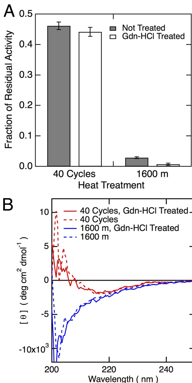
FIGURE 5. Effects of a denaturant on heat-inactivated anti-hCG VHH. A , the amount of residual activity after Gdn-HCl treatment was estimated and compared with that of VHH without Gdn-HCl treatment. Samples (40 \mu\text{M} ) were unfolded using a final concentration of \sim 6 M Gdn-HCl and then dialyzed against HBS-EP buffer without EDTA to remove the denaturant. Error bars represent S.D. B , comparison of CD spectra of heat-inactivated samples at 37 °C with or without \sim 6 M Gdn-HCl treatment followed by refolding. m , minutes; deg , degrees.
