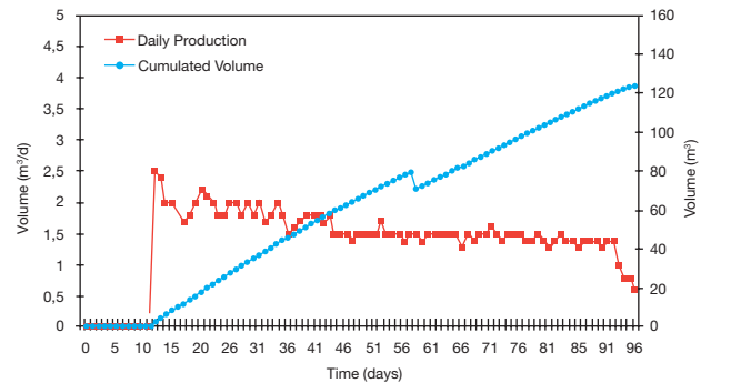
Figure 5. Kinetics and cumulative production of biogas during the cool season (20–30°C).
