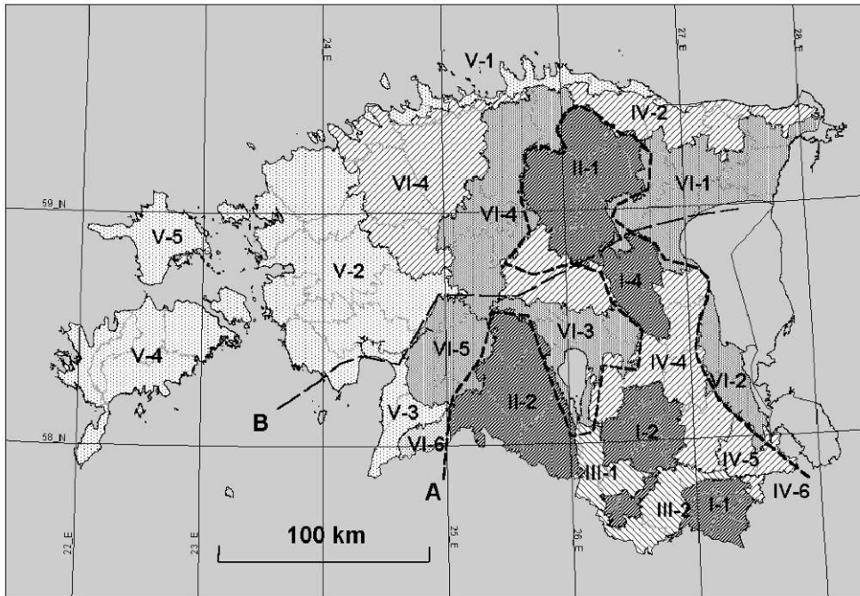
Figure 2. Typological landscape regions (modified from Arold, 2001).
