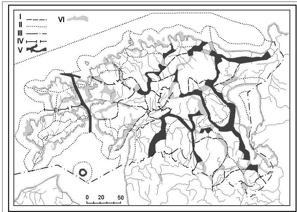
Figure 1. Landscape regions defined with the help of combinations of different borders.
