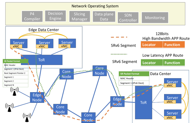
Fig. 1 Segment Routing Transportation in 5G network Edge Data Center to Core Data Center Architecture
