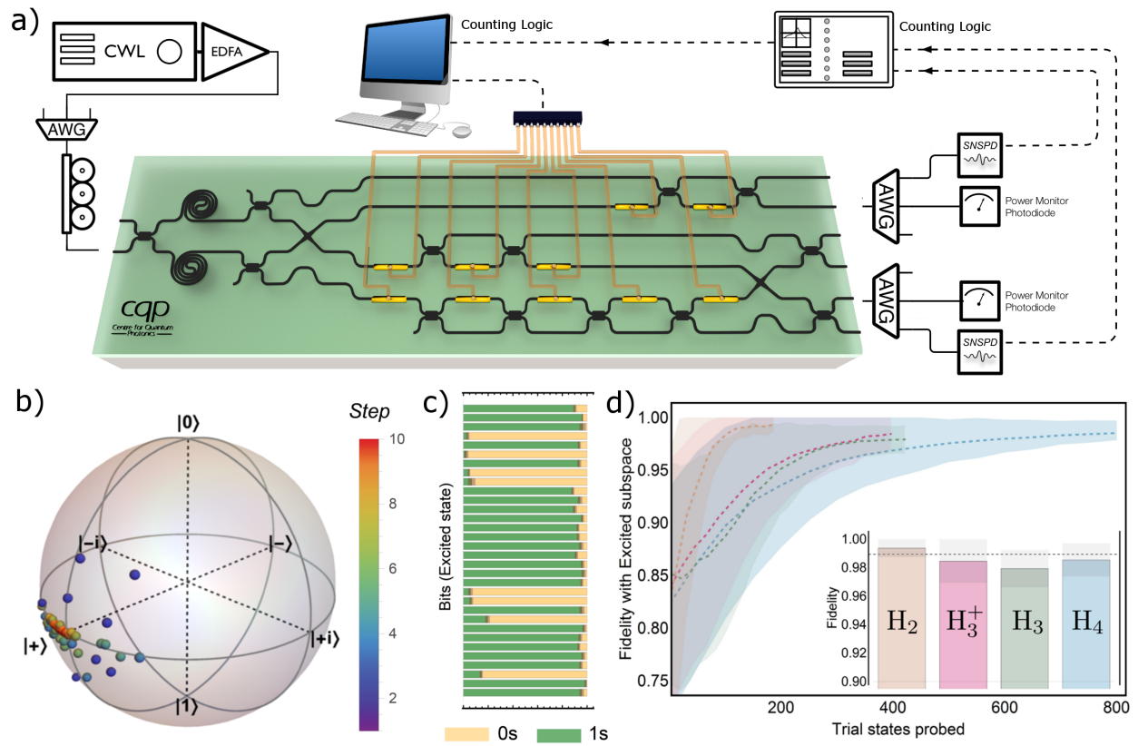
Fig. 1: a - Schematic of the 2 qubits device used to implement CU operations, along with basic off-chip components. b - Bloch sphere showing the evolution of trial input states |\phi_T\rangle , in different colors as per algorithm step, converging to the excited state |+\rangle for the experimentally investigated \hat{H} . c - Test IPEA run up to 32-bits, for the excited state found. The histogram bars provide experimental normalized coincidence counts, obtained from the projectors of |\phi_C\rangle on the computational basis. d - Simulated behaviour of the variational protocol in estimating excited states for test Hamiltonians of different size. Final fidelities achieved are emphasized in the inset with the same color-coding. Shaded areas indicate a 67.5% confidence interval.
