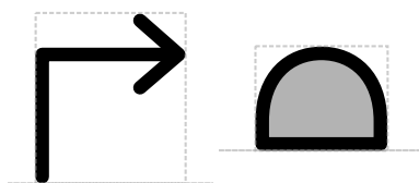
Figure 2: Examples of glyph specification: this specification for the sequence feature glyphs for Promoter (left) and Ribosome Entry Site (right) include the glyph outline, fill (grey center of Ribosome Entry Site), bounding box (dashed box), and recommended alignment with the nucleic acid backbone (dashed horizontal line), all at a preferred relative scale.
