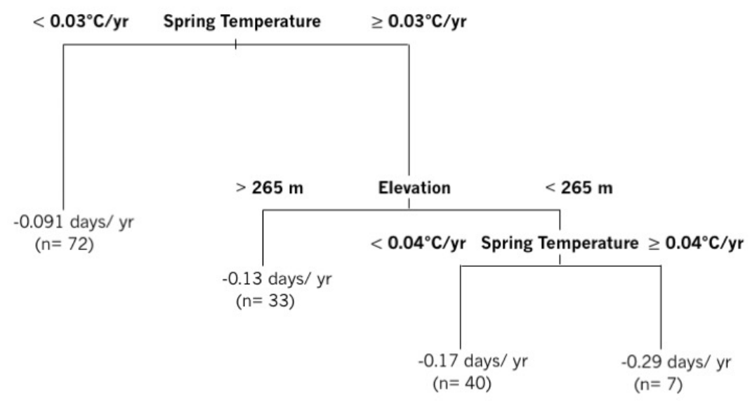
Figure 2: Drivers of global ice breakup trends from 1951-2014 identified using regression tree analysis. Trends in spring air temperatures and elevation explained 46% of the variation in ice breakup trends for 152 lakes across the Northern Hemisphere.
