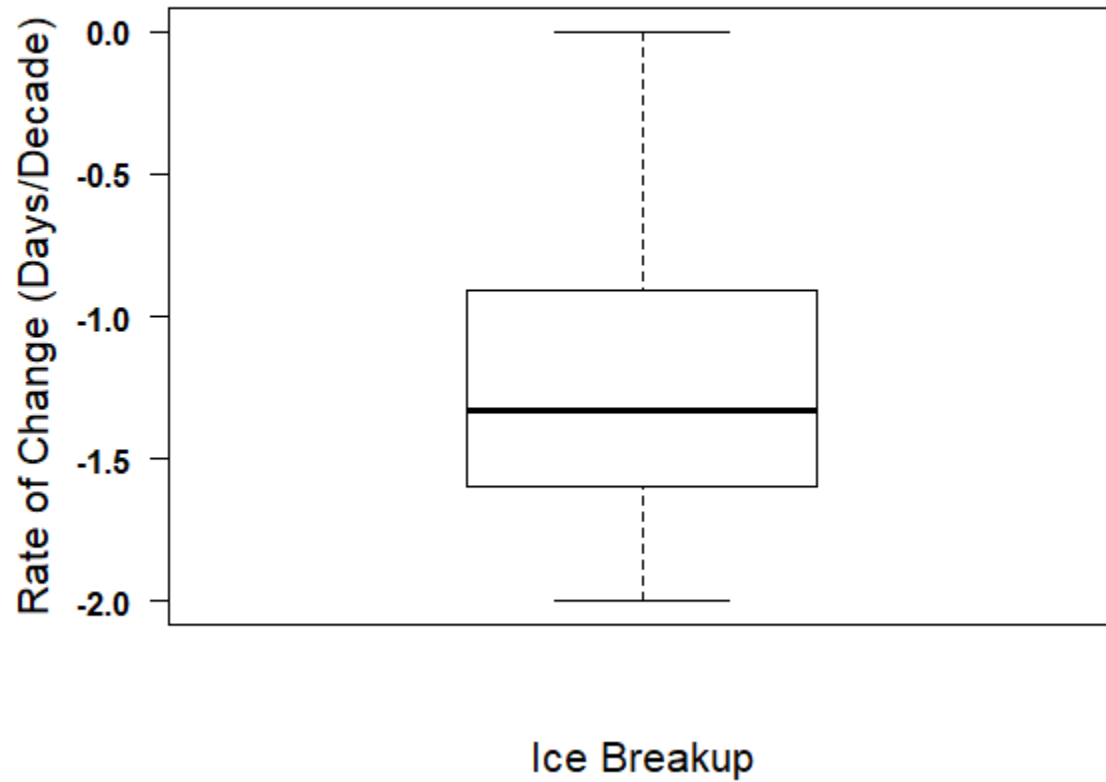
Figure 2. Rate of change of lake ice breakup (day of year) in nine north temperate lakes between 1981/2 and 2014/5.
