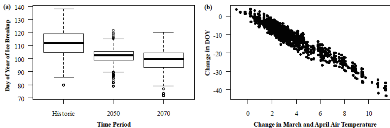
Figure 4. (a) The timing of lake ice breakup (day of year) for the historic period (1981/2–2014/5), and forecasted in 2050, and 2070; (b) Forecasted change in the day of ice breakup with the corresponding change in mean March–April air temperature ( ^{\circ}\text{C} ) under 126 projected climate scenarios.
