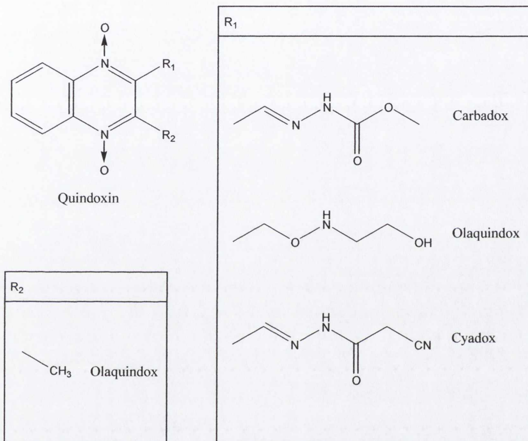
Fig. 1.3 Structures of QDN and its derivatives, CBX, OQX and cyadox.
