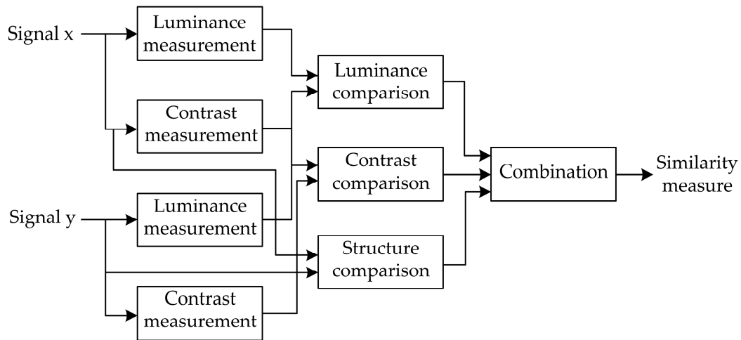
Figure 1. The block diagram of the SSIM index metric.
