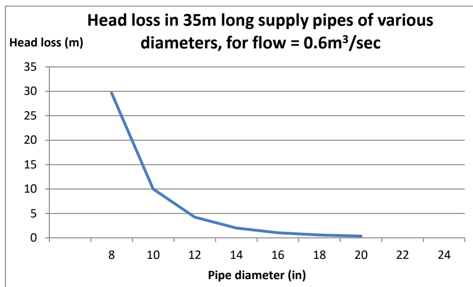
Figure 3-8. Head loss in 35m long (deep) pump intake pipe for (typical) flow of 0.6m 3 /sec
