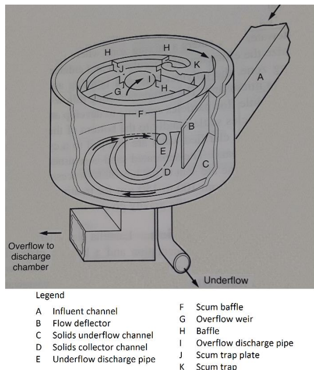
Figure A5.2: Diagram of swirl separator (aka vortex separator aka hydrocyclone) operation. Source: (Metcalf & Eddy Inc. 2004).
