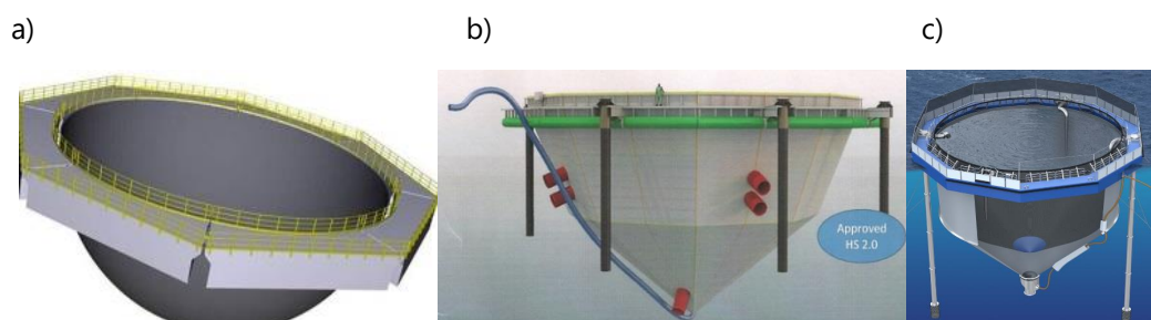
Figure 3-2. The geometries of the flexible containment systems of Akvadesign/Akvafuture (a), Botngaard (b) and Ecomerden (c)
