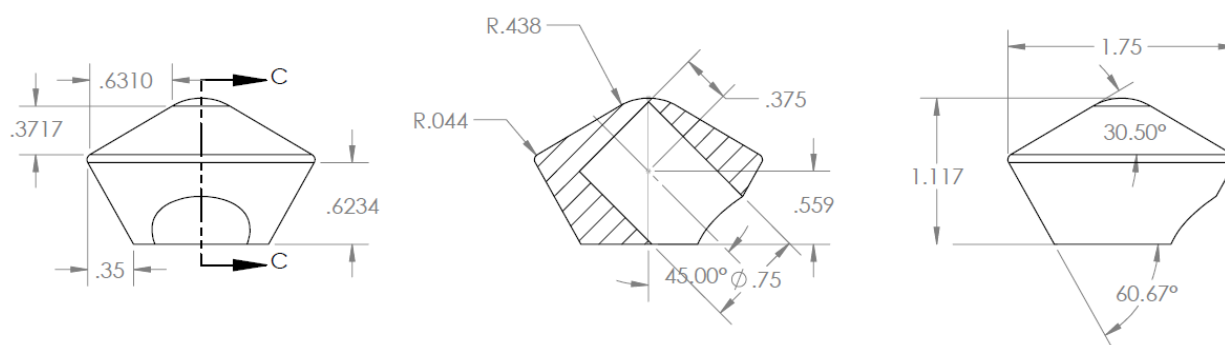
Figure 70: Drawing of 45° model for use with dummy sting. Dimensions in inches. Same external geometry as the 0° model; the internal cavity was rotated about the model centroid by 45°. Models at other orientations have a cavity rotated about the centroid by the desired angle.
