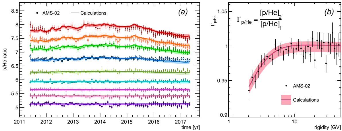
FIG. 3. (a) time profiles of the p/He ratio evaluated at rigidities \mathcal{R} = 2.2, 2.5, 2.8, 3.4, 5.1, 7.4, 10.5, 15, and 22 GV (from top to bottom); (b) rigidity dependence of the ratio \Gamma_{p/He} = [p/He]_{t_2}/[p/He]_{t_1} calculated for February 2014 ( t_1 ) and May 2017 ( t_2 ). In both plots, the new data from AMS are compared with model predictions and their uncertainties.
