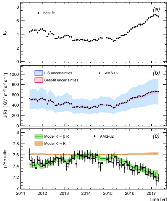
FIG. 2. (a) Time-series of the best-fit k_0 -values derived with the AMS proton data at \mathcal{R} = 1 - 60 GV [14]; (b) time profile of the proton flux measured by AMS at \mathcal{R} = 2 GV in comparison with calculations, LIS uncertainties and uncertainties from the fit; (c) measured time profile of the p/He ratio at \mathcal{R} = 2 GV in comparison with best-fit calculations for K = \beta \mathcal{R} (thick solid line) and K \propto \mathcal{R} (thin dashed line).
