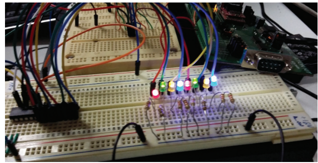
Figure 6: Tibbo evaluation card communicating with an MCP23S17 through an SPI channel. The Tibbo evaluation card is driven by DCS commands coming from the workstation.
