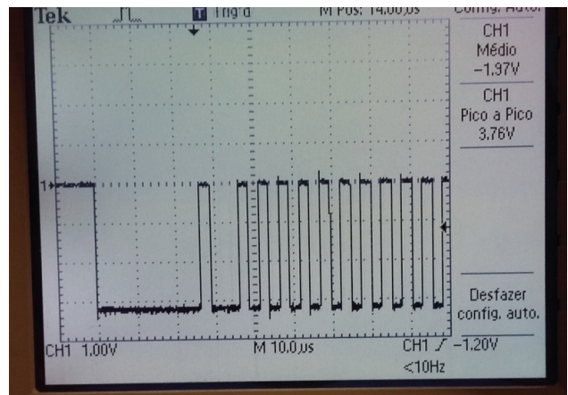
Figure 7: SPI signal (MOSI or SI) during communication. The transmission clock in the Tibbo was set to a period of about 5 \mu s (2 periods per oscilloscope division in this image).
