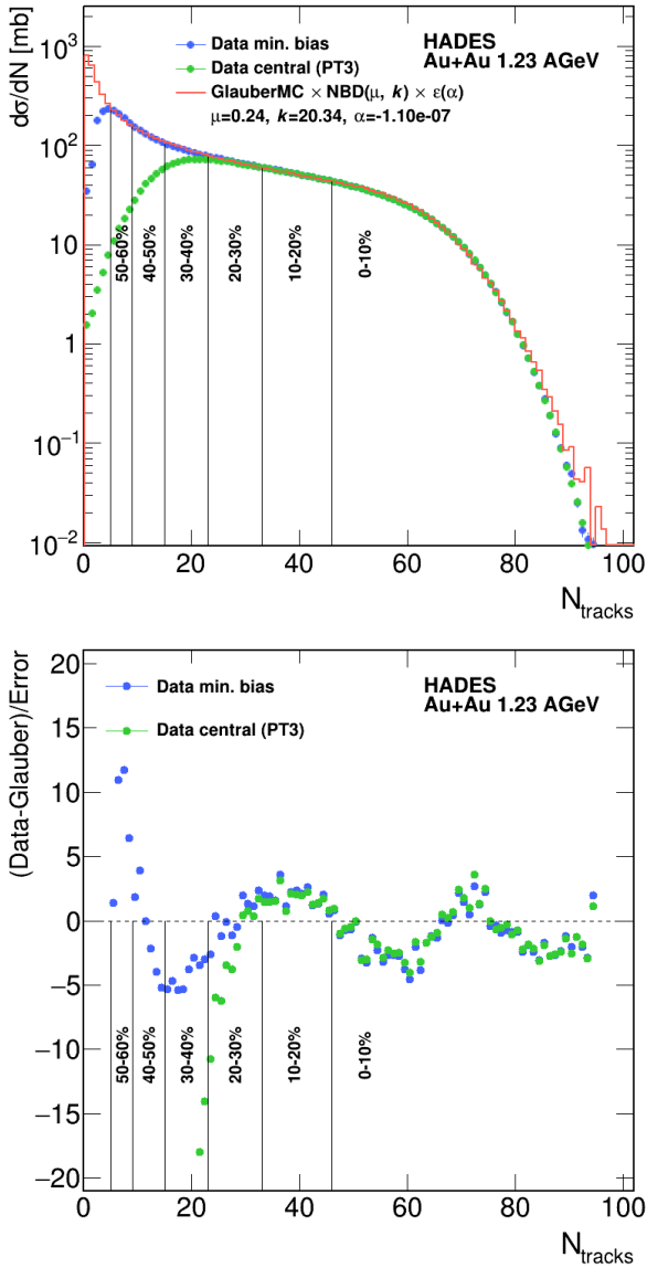
Fig. 2. Upper panel: The cross section as a function of N_{\text{tracks}} for minimum bias (blue symbols) and central (PT3 trigger, green symbols) data in comparison with a fit using the Glauber MC model (red histogram). The centrality classes are represented by the vertical lines. See text and table 1 for a description of the parameters \mu , k and \alpha . Lower panel: The difference between data and Glauber MC model divided by the quadratic sum of both errors.
