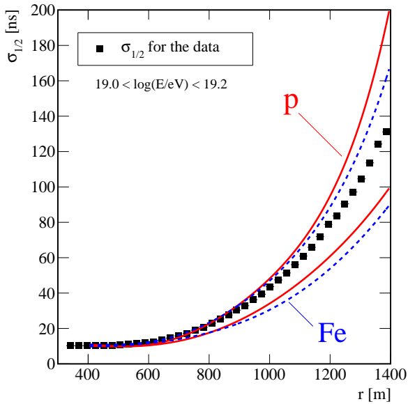
Figure 9: Risetime uncertainties estimated for protons (red lines), iron nuclei (blue dashed lines) and data as a function of core distance. For a clear view, the uncertainties corresponding to data are the average values. The uncertainties have been evaluated for events with energies in the range 19.0 < \log(E/eV) < 19.2 . The regions bracketed by the lines indicate the spread of the events simulated with QGSJETII-04 at a given distance.
