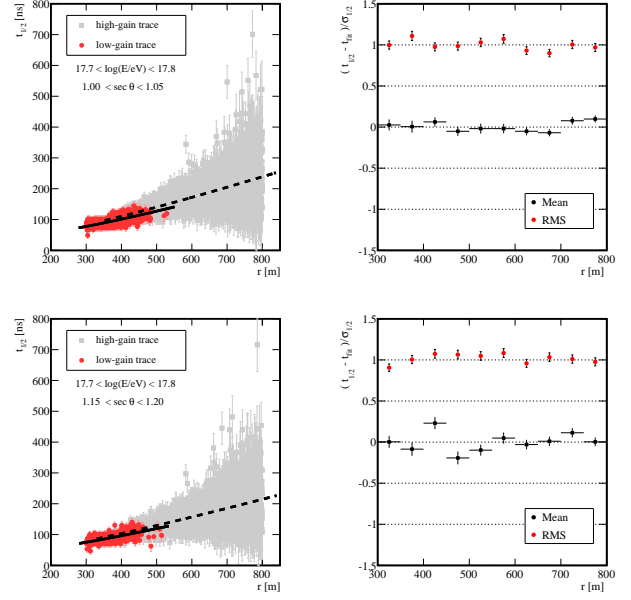
Figure 6: Examples of benchmark fit for the 750 m array. (Top panels) 1.00 < \sec \theta < 1.05 . (Bottom panels) 1.15 < \sec \theta < 1.20 . The solid (dashed) line corresponds to the fit done to the risetimes computed using the low-gain (high-gain) trace.
