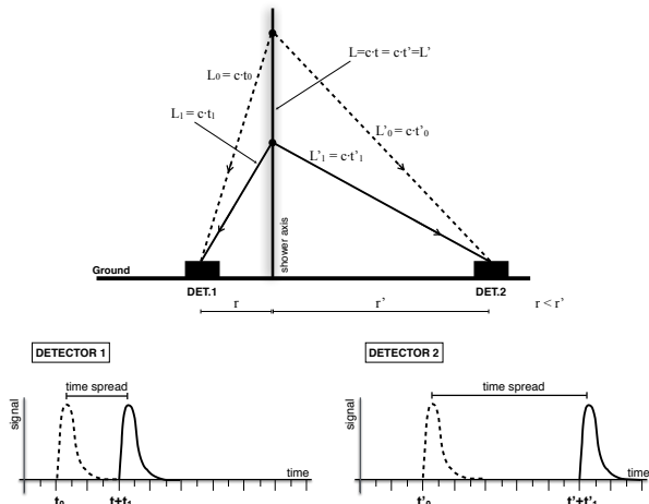
Figure 1: Qualitative sketch of how geometrical effects affect the temporal spread of the muons at a detector.
