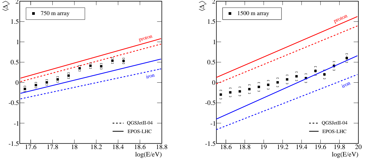
Figure 10: \langle \Delta_s \rangle as a function of the energy for the two surface arrays. Brackets correspond to the systematic uncertainties. Data are compared to the predictions obtained from simulations.
