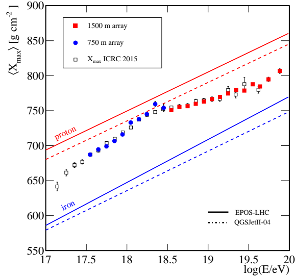
Figure 17: Evolution of \langle X_{\max} \rangle as a function of energy. The figure compares the mean values of the X_{\max} distributions measured by the fluorescence and surface detectors of the Pierre Auger Observatory. In most cases the uncertainties are smaller than the size of the symbols.
