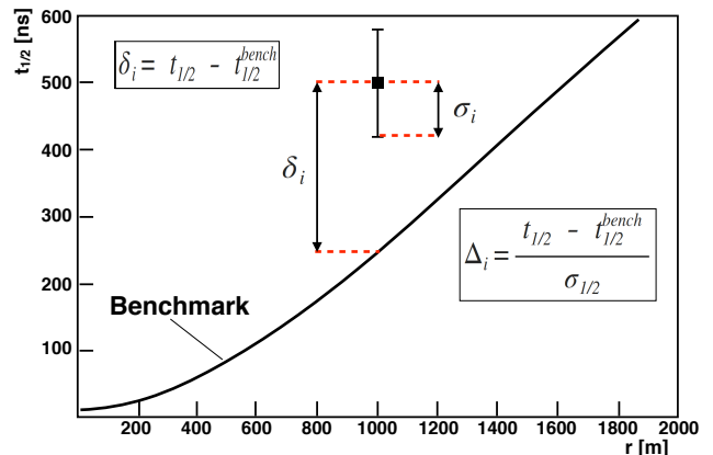
Figure 4: Schematic diagram to illustrate the Delta method.
