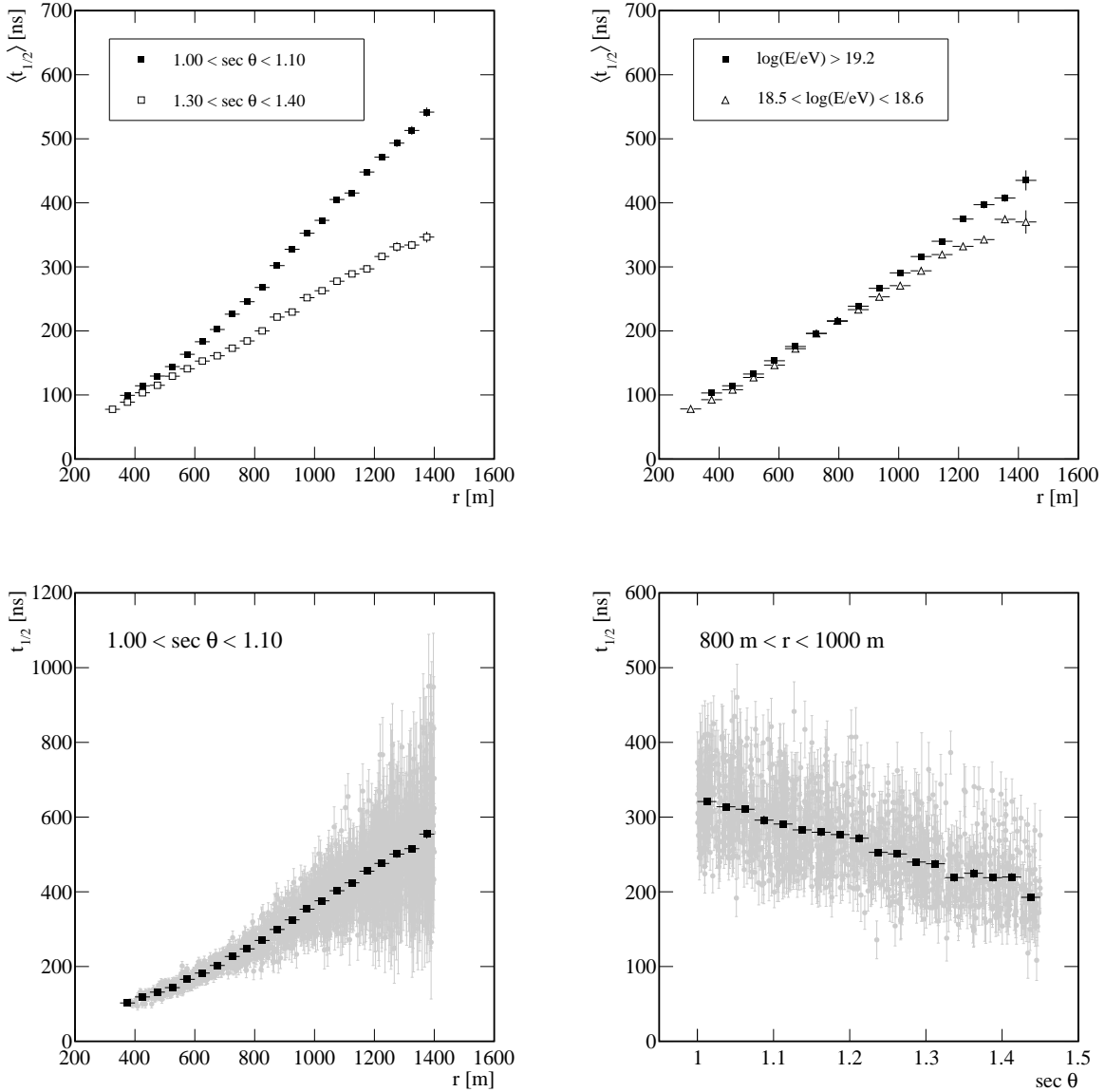
Figure 2: (Top left) The risetime as a function of distance to the shower core for two different intervals of \sec \theta in the energy range 19.0 < \log(E/eV) < 19.2 . (Top right) The risetime as a function of distance for two different energy bands in the angular range 1.20 < \sec \theta < 1.30 . (Bottom left) Illustration of the spread in the risetimes as a function of distance for events in the energy range 19.1 < \log(E/eV) < 19.2 . (Bottom right) Illustration of the variation of risetime with zenith angle for events in the energy range 19.1 < \log(E/eV) < 19.2 . All plots are based on experimental data
