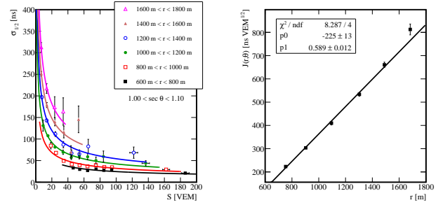
Figure 3: (Left) Uncertainty obtained with pair detectors as a function of the station signal for vertical events ( 1.00 < \sec \theta < 1.10 ). Each line is the result of the fits performed for different distance ranges. Each point represents the average measurements of at least 10 pair detectors. (Right) The parameter J(r, \theta) as a function of the distance to the core for the same zenith angle range.
