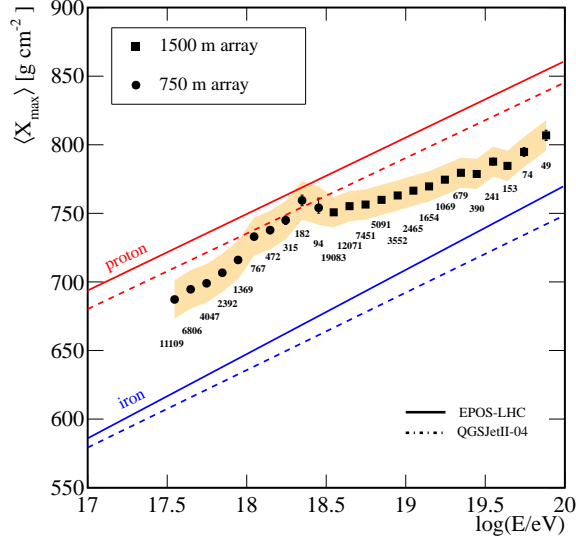
Figure 15: Mean values of the X_{\max} distributions obtained with the data of the 750 m and 1500 m surface arrays as a function of the energy. The shaded area indicates the systematic uncertainties. Data are compared to the predictions from simulations of protons and iron nuclei for two different hadronic models. The number of selected events in each energy bin is indicated.
