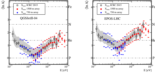
Figure 18: \langle \ln A \rangle as a function of the energy. QGSJetII-04 and EPOS-LHC have been used as the reference hadronic models. The results of the Delta method are compared with those based on X_{\max} measurements done with the FD [21]. Brackets and shaded areas correspond to the systematic uncertainties; bars correspond to uncertainties of statistical nature.
