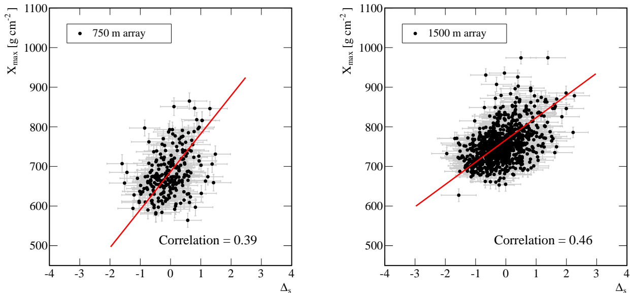
Figure 14: (Left) Correlation of X_{\max} and \Delta_s for the 252 events from the 750 m array. (Right) Correlation of X_{\max} and \Delta_s for the 885 events of the 1500 m array.
