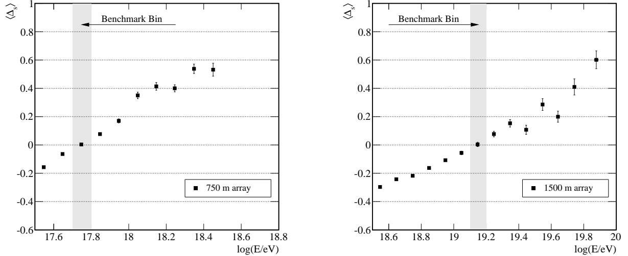
Figure 8: Evolution of \langle \Delta_s \rangle as a function of energy for the two surface arrays: 750 m (left), 1500 m (right). The grey bands show the energy ranges where the benchmark functions were defined.
