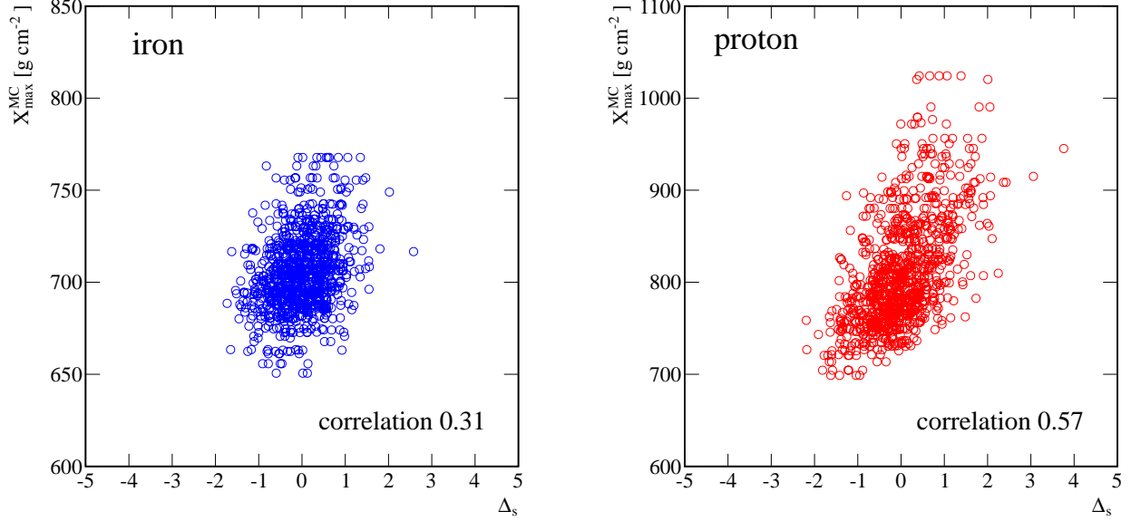
Figure 13: Pearson's correlation of \Delta_s and the true values of X_{\max} for events simulated with QGSJETII-04 in the energy range 19.1 < \log(E/\text{eV}) < 19.2 . The left panel corresponds to iron nuclei; the right panel shows the correlation for protons. Values of \Delta_s are computed for three stations.
