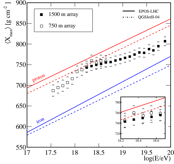
Figure 16: Same as Fig. 15 including additional X_{\max} measurements from the surface detectors above and below 3 EeV. (Inset) Three energy bins have been included below 3 EeV using the data of the 1500 m array and two measurements added above 3 EeV use the data of the 750 m array. There is good agreement between measurements in the overlap region. The brackets correspond to systematic uncertainties.
