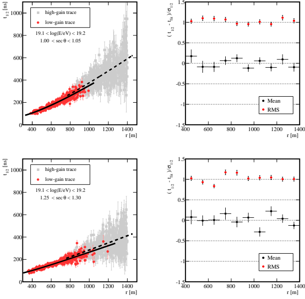
Figure 7: Examples of benchmark fit for the 1500 m array. (Top panels) 1.00 < \sec \theta < 1.05 . (Bottom panels) 1.25 < \sec \theta < 1.30 . The solid (dashed) line corresponds to the fit done to the risetimes computed using the low-gain (high-gain) trace.
