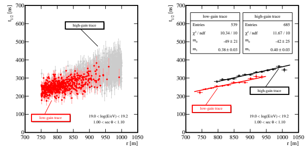
Figure 5: (Left) Risetimes as a function of core distance for events with and without saturation in the high-gain channel. We have selected events with energies 19.0 < \log(E/\text{eV}) < 19.2 and zenith angles 1.00 < \sec \theta < 1.10 . (Right) Same as left plot but this time we show average values to make more evident the difference between measurements when the saturation of the high-gain channel is present.
