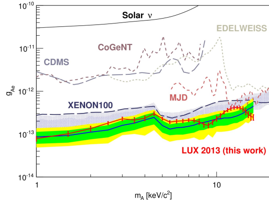
FIG. 7: Red curve: LUX 2013 data 90% C.L. limit on the coupling between galactic axion-like particles and electrons. Blue curve: 90% C.L. sensitivity, \pm 1 \sigma (green band), and \pm 2 \sigma (yellow band).
