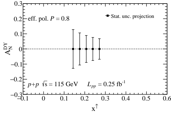
Fig. 6: Fast statistical projections for Drell-Yan A_N as a function of x^\uparrow with a ALICE-like detector. See text for details.
