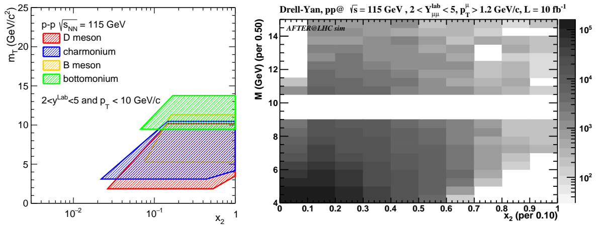
Fig. 2: Left panel: The range in the transverse mass m_T vs. parton momentum fraction x_2 accessible in AFTER@LHC in p + p collisions at \sqrt{s_{NN}} = 115 \text{ GeV} with J/\psi , \Upsilon and D-meson measurements. Right panel: the x_2 vs. Drell-Yan mass coverage. [Both are for a LHCb-like detector]
