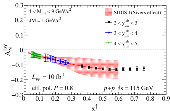
Fig. 5: Statistical projections for the Drell-Yan A_N measurement as a function of x^\uparrow with a LHCb-like detector. Note that the range in x^\uparrow is limited by the bin sizes in y and M . We have checked that measurements can probably be done with an accuracy of 5% up to x^\uparrow \approx 0.95 as expected from Fig. 2.
