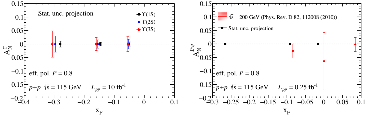
Fig. 3: Projections for \Upsilon (left panel) and J/\psi (right panel) A_N as a function of x_F for AFTER@LHC with a LHCb-like detector. For the J/\psi case, these are compared to existing data from PHENIX [12] in red.
