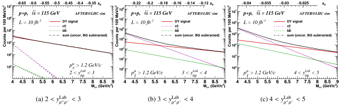
Fig. 1: Invariant mass distribution of the correlated \mu^+\mu^- pairs originating from Drell-Yan, c\bar{c} and b\bar{b} production for a LHCb-like detector. The uncorrelated background is estimated with the like-sign method and then subtracted from the overall simulated \mu^+\mu^- mass spectrum.
