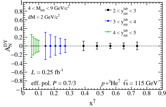
Fig. 7: Statistical projections for Drell-Yan A_N as a function of x^\uparrow in p+{}^3\text{He}^\uparrow collisions at \sqrt{s} = 115 \text{ GeV} .
