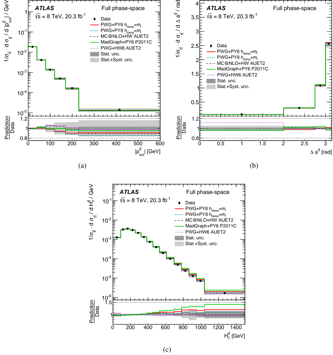
Figure 14: Full phase-space normalized differential cross-sections as a function of the (a) out-of-plane momentum ( |p_{\text{out}}^t| ), (b) azimuthal angle ( \Delta\phi^t ), and (c) scalar sum of the transverse momenta of the hadronic and leptonic top quarks ( H_T^t ) of the t\bar{t} system. The grey bands indicate the total uncertainty on the data in each bin. The POWHEG+PYTHIA generator with h_{\text{damp}} = m_t and the CT10nlo PDF is used as the nominal prediction to correct for detector effects.
