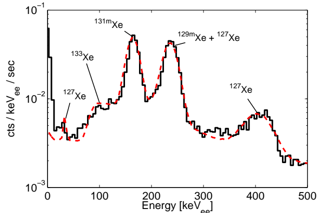
Figure 4: Early zero-field LUX data taken 12 days after bringing the Xe underground, featuring peaks from cosmogenically activated Xe isotopes. The measured spectrum is shown as the black histogram. The best-fit spectrum for cosmogenic Xe isotopes plus exponential background is shown as the dashed curve (gray in print, red online). The simulation spectrum is comprised of ^{127}\text{Xe} , ^{129m}\text{Xe} , ^{131m}\text{Xe} , and ^{133}\text{Xe} components, with decay rates of 2.7, 3.6, 4.4, and 3.6 mBq \text{kg}^{-1} respectively. Simulated peak resolution is measured from the ^{129m}\text{Xe} and ^{131m}\text{Xe} peaks and extrapolated as \sqrt{E} .
