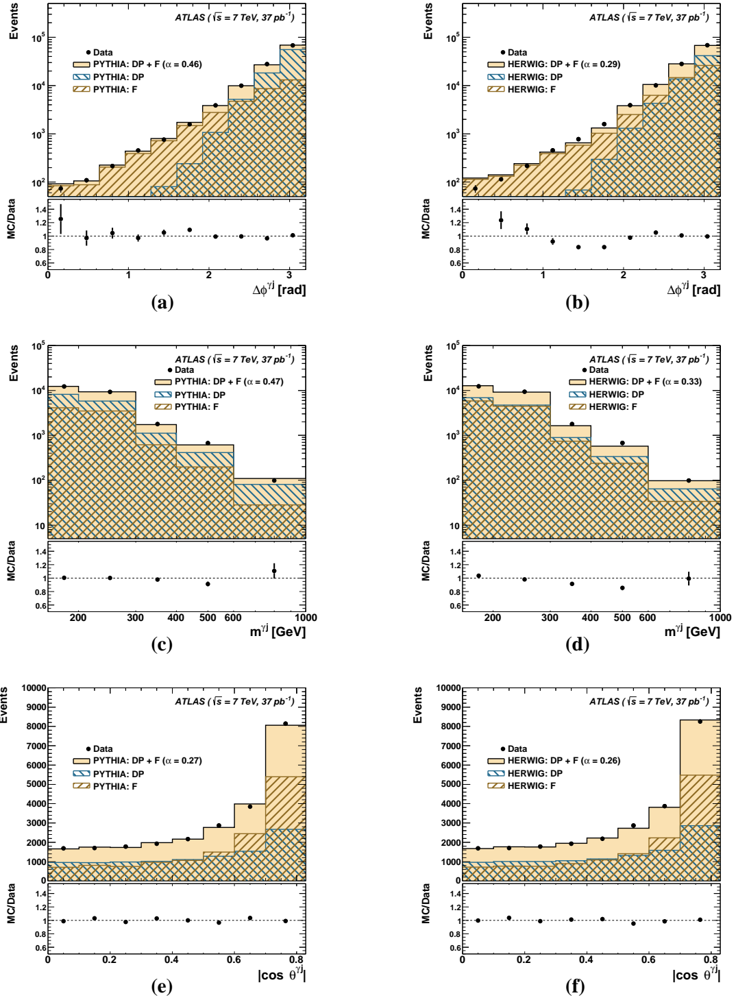
Figure 7: The estimated signal yield in data (dots) using the signal leakage fractions from (a,c,e) PYTHIA or (b,d,f) HERWIG as functions of (a,b) \Delta\phi^{j1} , (c,d) m^{j1} and (e,f) |\cos\theta^{j1}| . The distributions as functions of m^{j1} ( |\cos\theta^{j1}| ) include requirements on |\cos\theta^{j1}| ( m^{j1} ) and |\eta^\gamma + y^{\text{jet}}| (see text). Other details as in the caption to Fig. 6.
