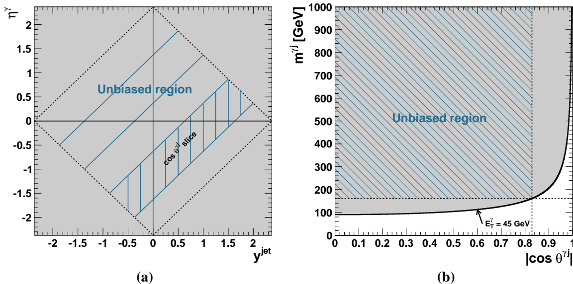
Figure 2: The selected regions in the (a) \eta^\gamma - y^{\text{jet}} and (b) m^\gamma - |\cos \theta^\gamma| planes. In (a), the dashed lines correspond to: \eta^\gamma + y^{\text{jet}} = 2.37 (first quadrant), \eta^\gamma - y^{\text{jet}} = 2.37 (second quadrant), \eta^\gamma + y^{\text{jet}} = -2.37 (third quadrant) and \eta^\gamma - y^{\text{jet}} = -2.37 (fourth quadrant). In (b), the horizontal (vertical) dashed line corresponds to m^\gamma = 161 GeV ( |\cos \theta^\gamma| = 0.83 ) and the solid line corresponds to E_T^\gamma = 45 GeV.
