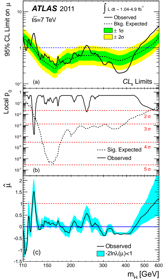
Figure 3: (a) The combined 95% CL upper limits on the signal strength as a function of m_H ; the solid curve indicates the observed limit and the dotted curve illustrates the median expected limit in the absence of a signal together with the \pm 1\sigma (dark) and \pm 2\sigma (light) bands. (b) The local p_0 as a function of the m_H hypothesis. The dashed curve indicates the median expected value for the hypothesis of a SM Higgs boson signal at that mass. The four horizontal dashed lines indicate the p_0 values corresponding to significances of 2\sigma , 3\sigma , 4\sigma and 5\sigma . (c) The best-fit signal strength as a function of the m_H hypothesis. The band shows the interval around \hat{\mu} corresponding to region where -2 \ln \lambda(\mu) < 1 .
