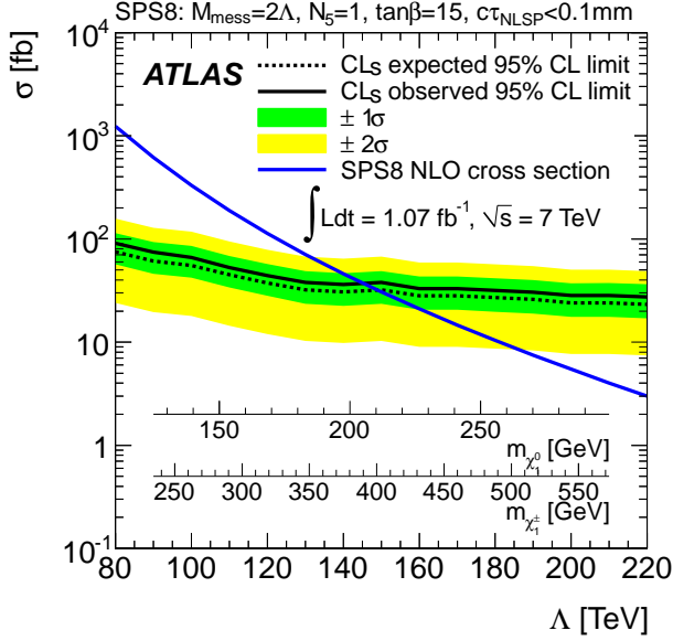
Figure 5: Expected and observed 95% CL upper limits on the sparticle production cross section in the SPS8 model, and the NLO cross section prediction, as a function of \Lambda and the lightest neutralino and chargino masses. Further SPS8 model parameters are M_{\text{mess}} = 2\Lambda , N_5 = 1 , \tan \beta = 15 , and c\tau_{\text{NLSP}} < 0.1 mm.
