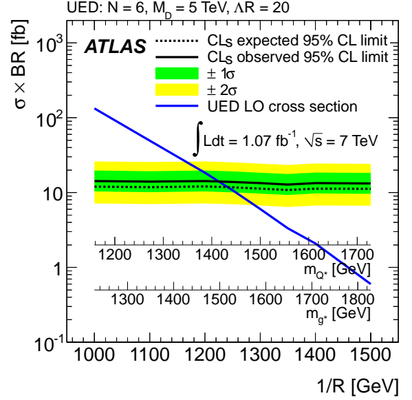
Figure 6: Expected and observed 95% CL upper limits on the KK particle production cross section times branching fraction to two photons in the UED model, and the LO cross section prediction times branching fraction, as a function of 1/R and the KK quark ( Q^* ) and KK gluon ( g^* ) masses. The UED model parameters are N = 6 , M_D = 5 TeV, and \Delta R = 20 .
