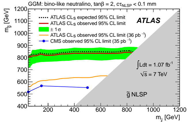
Figure 4: Expected and observed 95% CL lower limits on the gluino mass as a function of the neutralino mass in the GGM model with a bino-like lightest neutralino NLSP (the grey area indicates the region where the NLSP is the gluino, which is not considered here). The other sparticle masses are fixed to \sim 1.5 TeV. Further model parameters are \tan\beta = 2 and c\tau_{\text{NLSP}} < 0.1 mm. The previous ATLAS [1] and CMS [51] limits are also shown.
