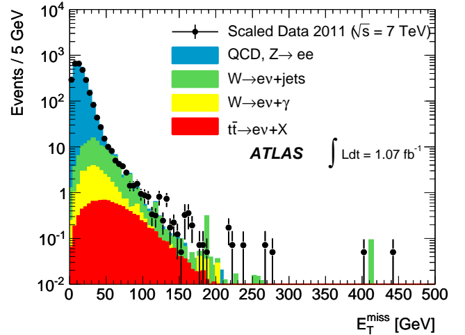
Figure 3: E_T^{\text{miss}} spectrum for the electron-photon control sample in data (points, statistical uncertainty only), normalised according to the probability for an electron to be mis-reconstructed as a tight photon, compared to the expected backgrounds displayed by components (stacked histograms). For the purpose of this comparison, the expected contributions from W(\rightarrow e\nu) + \text{jets}/\gamma and t\bar{t}(\rightarrow e\nu) + \text{jets} events are taken from MC simulation.
