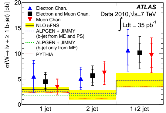
Figure 5: Measured fiducial cross section with the statistical (inner error bar) and statistical plus systematic (outer error bar) uncertainty in the electron, muon, and combined electron plus muon channel. The cross section is given in the 1, 2, and 1+2 jet exclusive bins. The measurements are compared with NLO [14] predictions. The yellow (shaded) band represents the total uncertainty on the prediction obtained by combining in quadrature the renormalisation and factorization scale, PDF set, and non-perturbative correction uncertainties. The leading order predictions from ALPGEN interfaced with HERWIG and JIMMY are given for b -jets generated only by the matrix element and by the matrix element and the parton shower. The prediction from PYTHIA is also shown.
