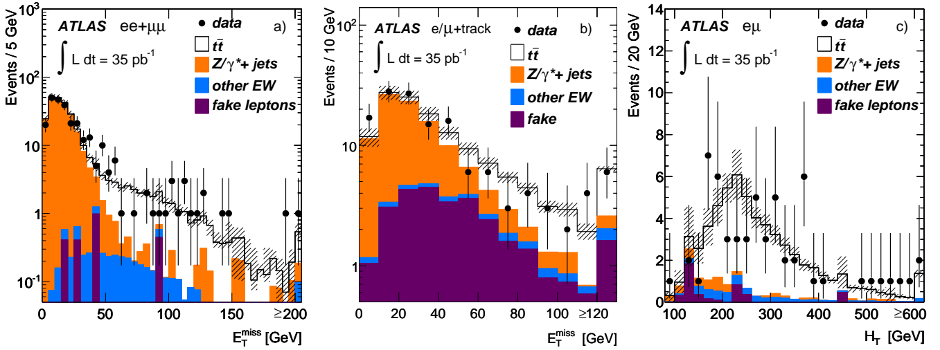
Figure 2: The E_T^{\text{miss}} distribution in the signal region without the E_T^{\text{miss}} > 40 \text{ GeV} requirement (a) for the ee and \mu\mu channels and (b) for the lepton+track channels. Fake denotes the contribution from fake track-leptons. The H_T distribution in the signal region for the e\mu channel is shown in (c) without the H_T > 130 \text{ GeV} requirement. Contributions from diboson and single top events are summarized as ‘other EW’. In all figures the last bin contains the overflow. The uncertainty on the data points are statistical uncertainties only, whereas the uncertainty bands include statistical and systematic uncertainties.
